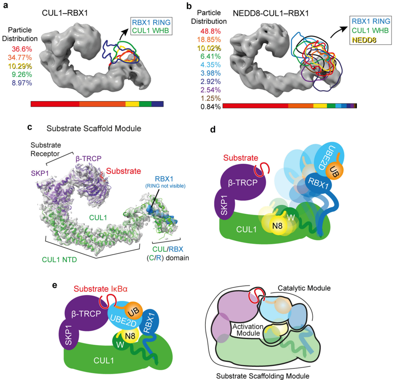
Extended Data Figure 2. CRL1 \beta -TRCP RBX1 RING and CUL1 WHB domains, without or with a covalently-linked NEDD8, are dynamic in the absence of other factors and are harnessed in catalytic architecture for substrate ubiquitylation with UBE2D.
