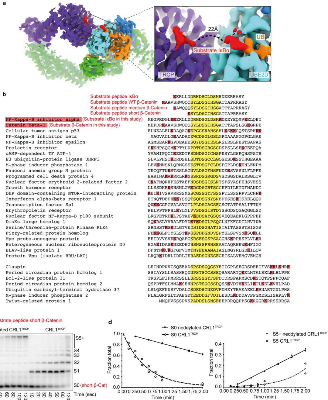
Extended Data Figure 6. Geometry between phosphodegron and acceptor in structure, substrates, and ubiquitylation.
