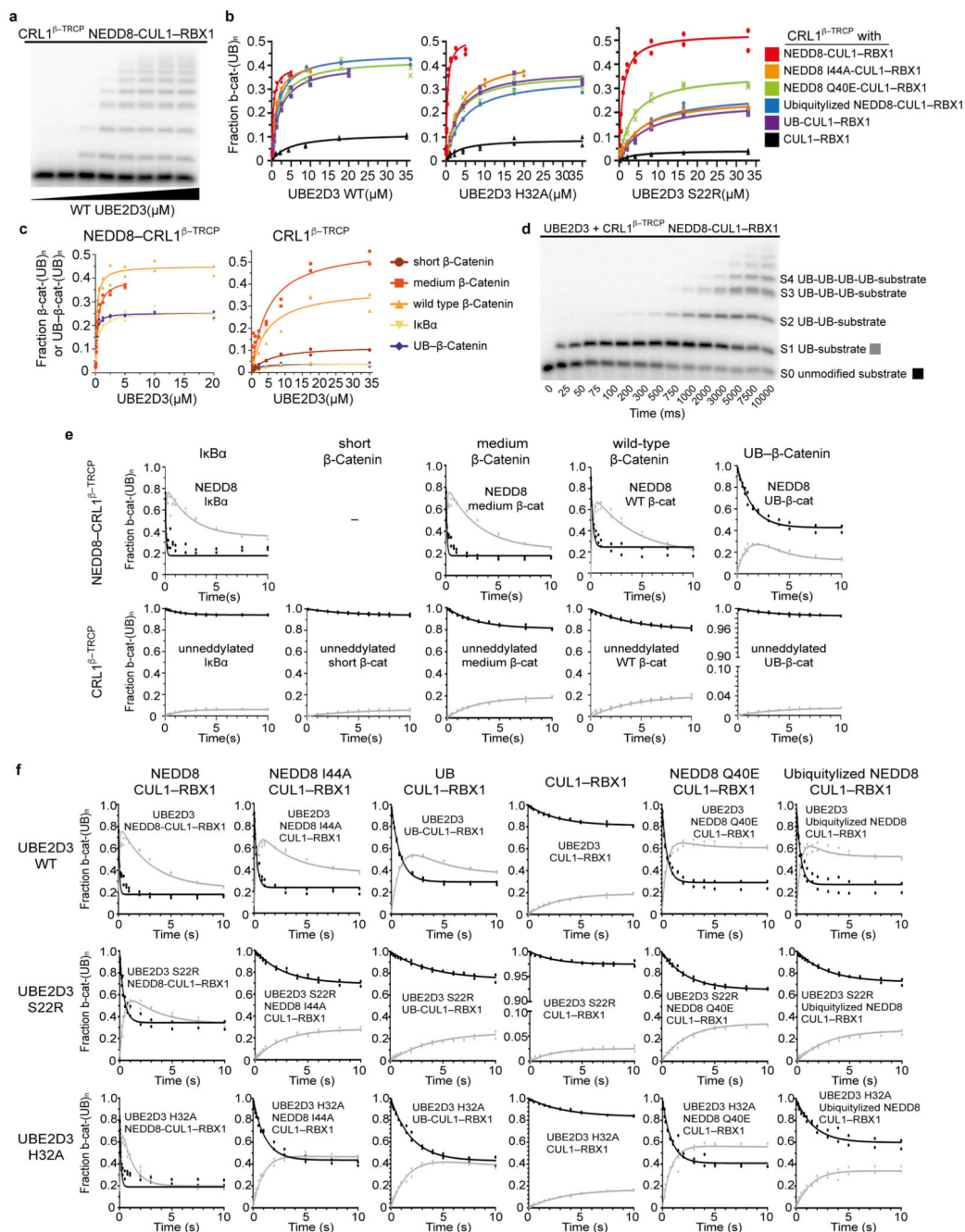
Extended Data Figure 1. Quantitative pre-steady state enzyme kinetics of neddylated CRL1 β-TRCP - and UBE2D-dependent ubiquitylation.
