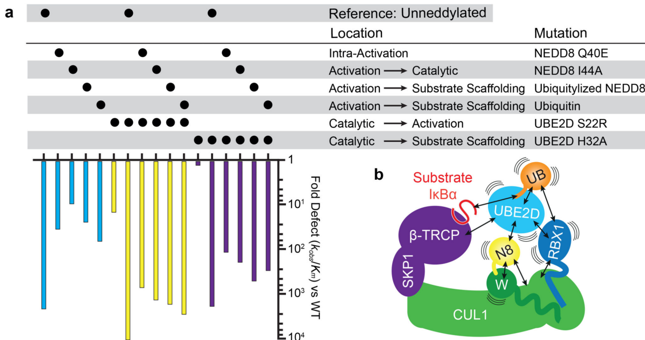
Figure 4. Multifarious interactions configuring rapid substrate priming
