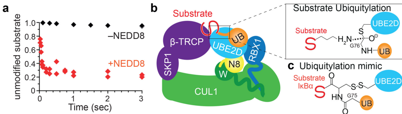
Figure 1. Role of NEDD8 and strategy to visualize dynamic ubiquitin transfer from E2 UBE2D to substrate by neddylated CRL1 \beta -TRCP
