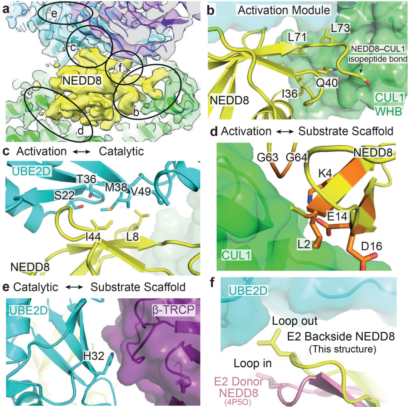
Figure 3. Intra- and inter-module interfaces specifying catalytic architecture for ubiquitin priming of substrate by neddylated CRL1 β-TRCP with UBE2D
