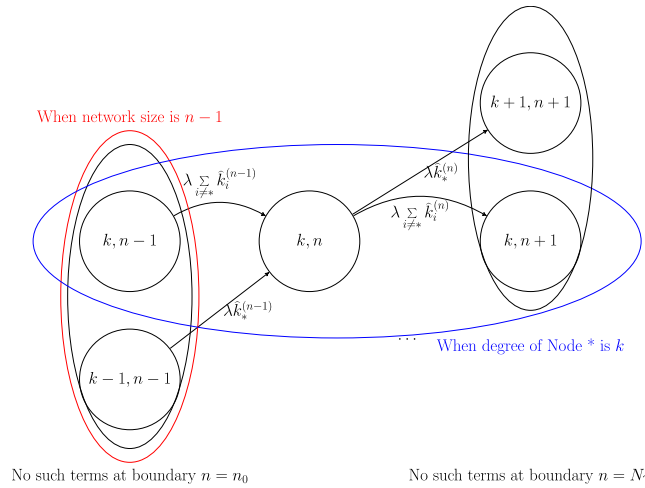
Figure 4. The state transition rate diagram of a two-dimensional Markov chain for a specific node *— where k denotes its degree and n denotes the network size that this node * is in, with values n_0 and N_T respectively at its initial time and time \mathcal{T} . In the diagram, it is noted that \hat{k}_*^{(n-1)} = k - 1 when k_*^{(n-1)} = k - 1 , and \hat{k}_*^{(n)} = \hat{k} when \hat{k}_*^{(n)} = k .
