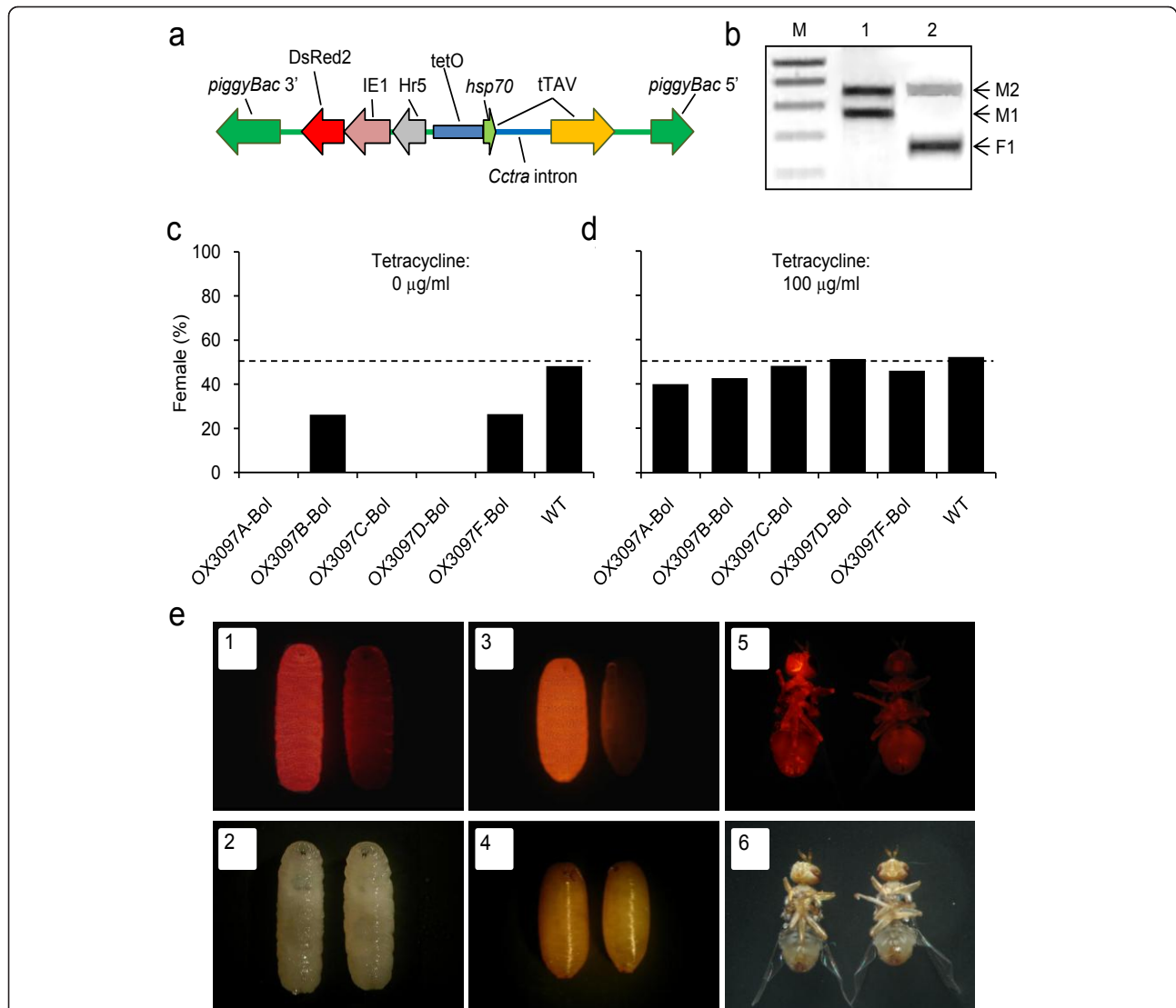
Figure 1 The OX3097 transposon and induced phenotypes in olive fly. (A) Diagrammatic representation of the OX3097 transposon. OX3097 comprises a fluorescent marker ( hr5-IE1-DsRed2 ), and the female-specific tTAV expression system ( tetO-Dm hsp70 minimal promoter - Cctra:tAV ) [15]. Sex-specific alternative splicing of the Cctra intron leads to production of tTAV and the initiation of a lethal tTAV positive-feedback loop in females only [14,15,34]. (B) Products of alternative splicing of Cctra:tAV in (lane 1) male and (lane 2) female OX3097D-Bol olive flies. Three splice variants were detected, corresponding to Cctra transcripts M1, M2 and F1 [18] (identity confirmed by sequencing). Only females produce the F1 splice variant, corresponding to the reconstitution of the tTAV open reading frame and leading to production of functional tTAV. Lane M shows DNA size standards: 200-1,000 bp in 200-bp increments (Eurogentec Smartladder). (C) Penetrance and (D) tetracycline repressibility of female lethality in five OX3097 olive fly lines. Strains OX3097A-D-Bol & F-Bol are five insertion lines of OX3097 in olive fly. Penetrance and repressibility of female-specific lethality was assessed by crossing heterozygous males of each strain to virgin wild-type (WT) females, and collecting eggs on filter paper saturated with water containing either 0 µg/ml tetracycline or 100 µg/ml tetracycline. The sex ratio of adult progeny expressing the DsRed2 fluorescent marker is shown for each strain compared with wild-type (WT) progeny. Lines A, C and D showed fully penetrant female-specific lethality when reared in the absence of tetracycline (off-tet); that is, they produced no female progeny off-tet in this assay. In lines C and D, female-specific lethality was also efficiently repressed on-tet. (E) Fluorescence microscopy allows discrimination of OX3097D-Bol from wild type at larval, pupal, and adult stages. Photomicrographs of OX3097D-Bol and wild-type olive flies under (upper panels) fluorescence and (lower panels) bright-field illumination. Each panel shows OX3097D-Bol to the left and wild-type to the right: OX3097D-Bol and wild-type (1,2) larvae, (3,4) pupae, and (5,6) adults are shown. Expression of DsRed2 is clearly visible all over the OX3097D-Bol larvae and pupae, and in areas of less opaque cuticle (for example, the labellum, upper thorax, leg joints, and anus) of OX3097D-Bol adults.
