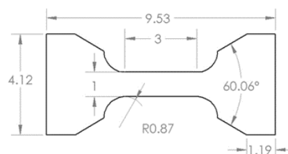
Figure 2. Dimension of the miniature tensile specimen. Units are in mm.
