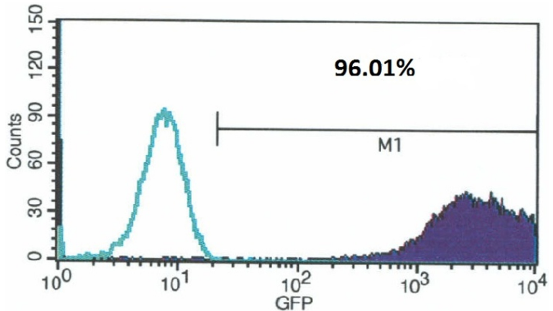
Fig 3. Within the histogram of GFP-transfected cells, the green line shows non-transfected cells and the region(M1) to the right of the vertical line represents the GFP fluorescence. The transfection efficiency and mean expression level can then be calculated by the CellQuest Pro Software.
