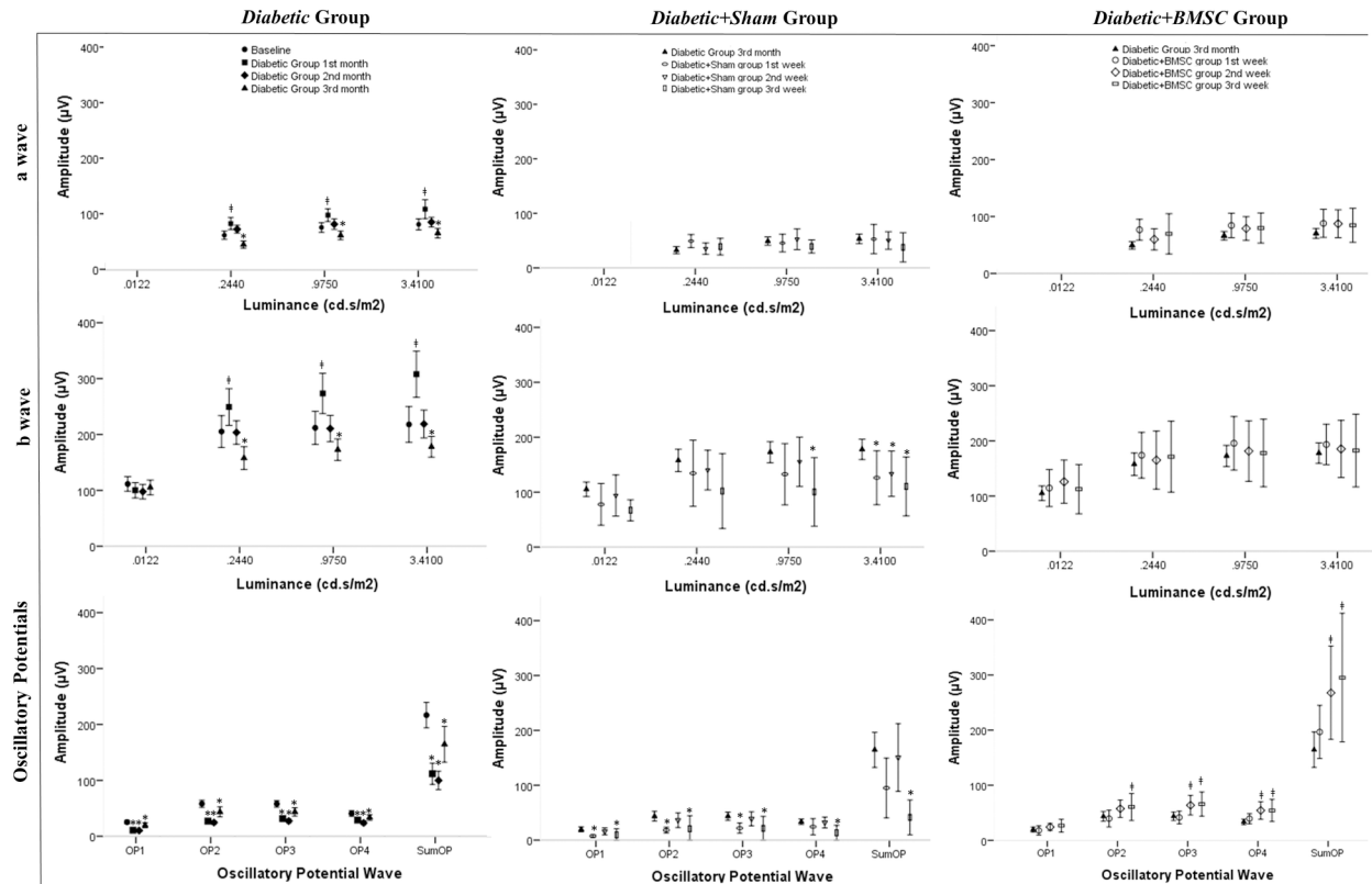
Fig 7. The graph representing the ERG amplitudes of Diabetic group at 1 st , 2 nd and 3 rd months compared to baseline and Diabetic+Sham and Diabetic+BMSC groups at 1 st , 2 nd and 3 rd weeks of injection compared to the Diabetic group at 3 rd month of induced diabetes. ‡, significantly more than the mean amplitude of the Baseline Group *, Significantly less than the mean amplitude of the Baseline Group OP1, Oscillatory Potential Wave 1; OP2, Oscillatory Potential Wave 2; OP3, Oscillatory Potential Wave 3; OP4, Oscillatory Potential Wave 4. SUMOP, The sum of all OP waves at measurement.
