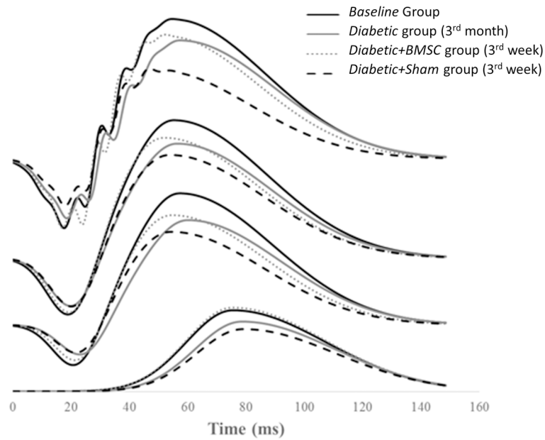
Fig 9. The plotted mean ERG waveforms at increasing light intensities of the Baseline group, Diabetic group (at 3 rd month), Diabetic+BMSC and Diabetic+Sham groups (3 rd week). BMSC, Bone marrow derived mesenchymal stem cells. Sham, in this study 2 \mu L of balanced salt solution was injected intravitreally as Sham.
