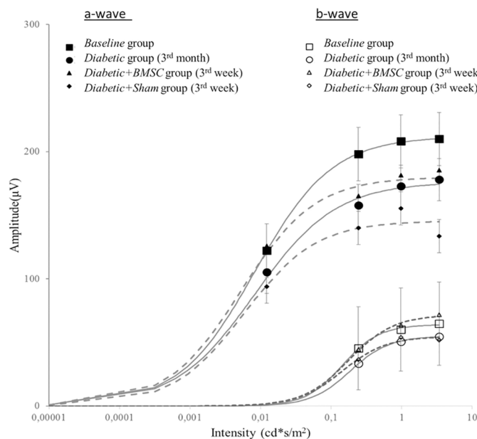
Fig 8. The representative mean intensity-response function of the “a” and “b” waves of the Baseline group, Diabetic group (at 3 rd month), Diabetic+BMSC and Diabetic+Sham groups (at 3 rd week). †, significantly more than the mean amplitude of the Baseline Group; BMSC, Bone marrow derived mesenchymal stem cells. OP1, Oscillatory Potential Wave 1; OP2, Oscillatory Potential Wave 2; OP3, Oscillatory Potential Wave 3; OP4, Oscillatory Potential Wave 4. SUMOP, The sum of all OP waves at measurement.
