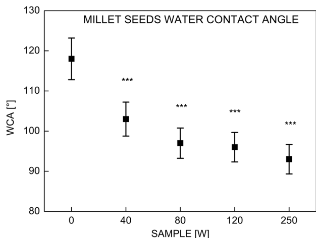
Fig. 8. Apparent water contact angle. Values are the arithmetic mean \pm SD. The significance was determined against untreated samples (0 W). Results were significant at *P < 0.05 ; **P < 0.01 ; ***P < 0.001 , n = 20 .
