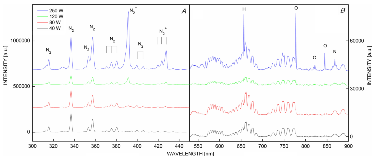
Fig. 2. Optical emission spectra of plasma discharge. (A) Range of spectra 300–450 nm containing dominant N_2 second positive system and N_2^+ first negative system; (B) range of spectra 525–900 nm containing atomic oxygen peaks. Both spectra were normalized to 1,000-ms integration time.
