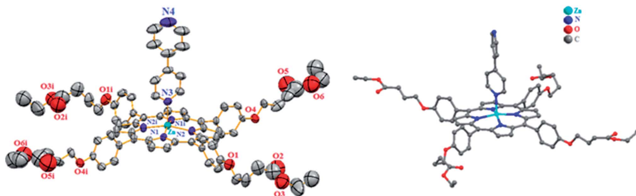
Fig. 3 The coordination environment of Zn(II) and structure conformation of [\text{Zn}(\text{TEBOP})(4,4'\text{-bpy})] . Ellipsoids are drawn at 30% probability. Symmetry codes are (i) = -x + 1, y, -z + 3/2 .
