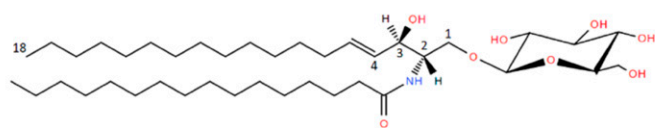
Glc-Cer(1) 18:1(4E);3OH[R]/16:0[2S]
