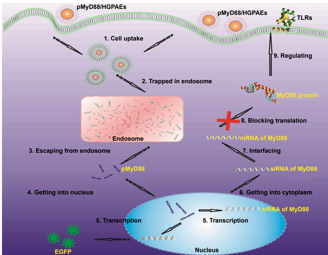
Figure 13 The functional mechanism of the pMyD88/HGPAE complex. Notes: After being entrapped by the acidic endosome, the pMyD88/HGPAE complex became swollen and disassembled. Then the pMyD88 escaped from the endosome and got into the nucleus to transcribe siRNA of MyD88 for suppressing the expression of MyD88 . Abbreviation: HGPAE, histidine-grafted poly(β-amino ester).
