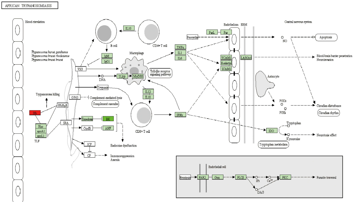
Figure 8 Schematic diagram of the proteins and metabolites pathways between HCCT-LC vs DCT and HCCT-LC vs HCCT-NLC. (A) Vitamin B6 metabolism. (B) Pentose and glucuronate interconversions metabolism. (C) African trypanosomiasis. Green means that the expression of proteins and metabolites is down-regulated and red means up regulated, the FDR-adjusted p -values were less than 0.001.
