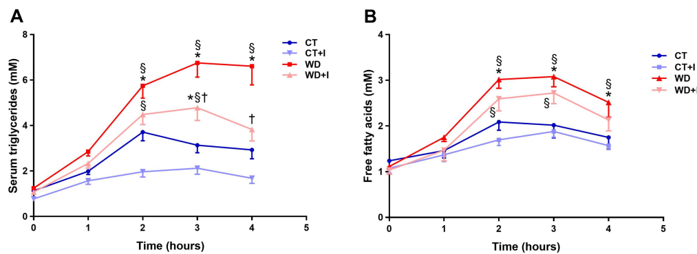
Figure 2. Serum triglyceride profile after olive oil load (A). Free fatty acid profile after olive oil load (B). Data are presented as mean ± SEM and analyzed with a mixed model ANOVA followed by Tukey post hoc tests. * p < 0.05 versus CT, § p < 0.05 versus CT + I, † p < 0.05 versus WD.
