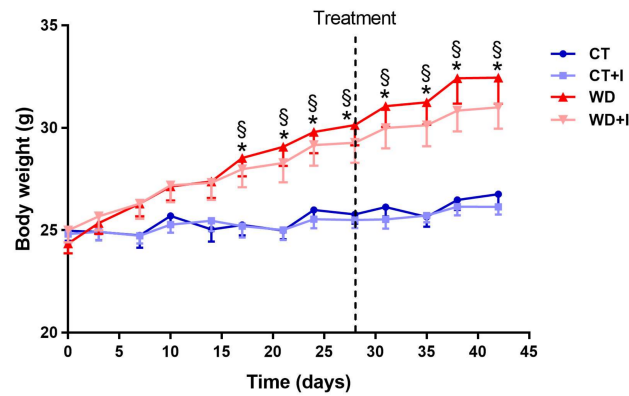
Figure 1. Body weight evolution. Inulin supplementation was introduced after 4 weeks. Data are presented as mean ± SEM and analyzed with a mixed model ANOVA followed by Tukey post hoc test. * p < 0.05 versus CT, § p < 0.05 versus CT + I.
