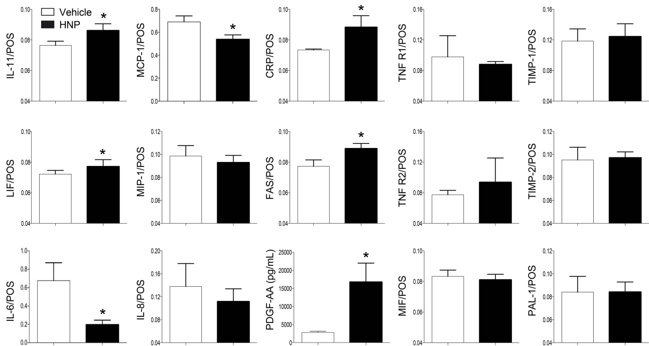
Figure 3 Changes of secretome profiles by MSCs after stimulation with PBS (Vehicle) or HNP at 10 µg/mL for 24 hrs. The cell culture supernatants were added in antibody-coated array membranes and incubated overnight at 4°C. Signal was detected by chemiluminescence after biotinylated antibody and horseradish peroxidase-conjugated streptavidin interactions. Quantification of protein expression was compared between Vehicle and HNP-treated groups (n=3). Expression of 6 out of 14 proteins detected reached statistical difference. Levels of PDGF-AA were measured by human-specific ELISA (n=17). *p < 0.05 vs Vehicle.
