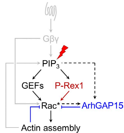
Figure 9. Model for PIP 3 -driven Rac regulation. The Rac GEF P-Rex1 (red connector) is the major (though not only) PIP 3 -activated Rac GEF. Downstream of Rac*, actin polymerization and ArhGAP15 function in parallel pathways (blue connectors) to inhibit Rac*. ArhGAP15 activity may require Rac* or be stimulated independently (black dashed arrows). Our data and previous studies are consistent with ArhGAP15 functioning in a negative feedback loop and/or an incoherent feedforward loop to regulate Rac (Costa et al., 2007; Radu et al., 2013). These interactions are masked by additional feedback and redundancy (gray arrows) when input is delivered at the level of the chemoattractant receptor but are revealed when input is delivered at the level of PIP 3 production via optogenetics (red lightning bolt).
