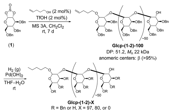
Scheme 1 Synthesis of Glcp-(1-2) -based adhesives. Glcp-(1-2) with X\% benzylation is abbreviated as Glcp-(1-2)-X .
