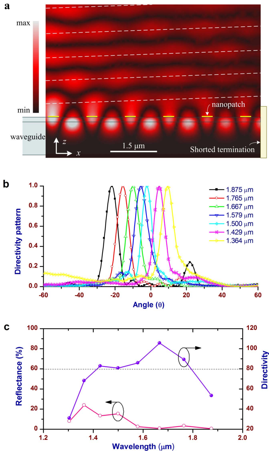
Figure 2 | Results of the proposed nanopatch array. (a) Magnetic field distributions in the central plane at the wavelength of 1.5 \mu\text{m} . The central plane is the one parallel to the xz plane and passing through the bottom line of the groove, with respect to which the proposed array is symmetric. Power emissions by the nanopatch antennas are clearly seen. The field intensity is gradually decreased along the x axis mainly due to the power emission. At the end of the CWPWG, the left small part of power (less than 3% of the excitation power for the array with 10 rows of nanopatch antennas) is terminated to avoid direct emission towards the x -axis direction. (b) Normalized directivity patterns of the nanopatch array at different wavelengths. For wavelengths from 1.364 to 1.875 \mu\text{m} , the beam is pointed from 9.5^\circ to -22^\circ . The average beam shifting gradient, beam shifting range over wavelength bandwidth, is around 6.2^\circ/100 \text{ nm} . (c) Reflectance observed in a reference plane of the CWPWG, 1.6 \mu\text{m} far from the first row of nanopatch antennas, and the peak directivity of the proposed nanopatch array. The maximum reflectance of around 23% occurs at 1.364 \mu\text{m} , and the reflectance is below 3.5% as the wavelength is over 1.579 \mu\text{m} . The peak directivity is above 80 from 1.429 to 1.765 \mu\text{m} , with a maximum of 105.7 at 1.667 \mu\text{m} .
