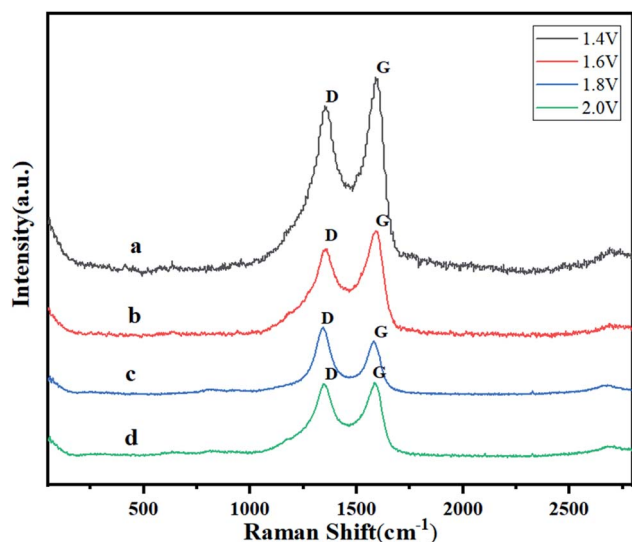
Fig. 6 Raman spectra of GR electrodes potentiostatic treated at (a) 1.4 V, (b) 1.6 V, (c) 1.8 V, and (d) 2.0 V.
