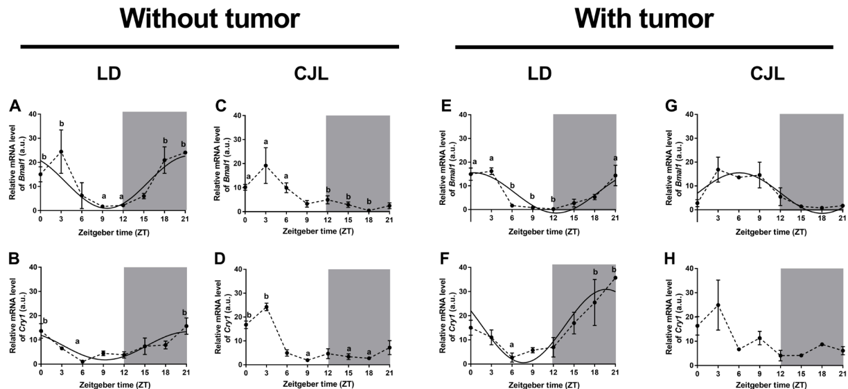
Fig. 4. Rhythms of clock genes in liver under the CJL schedule. Mean \pm SEM of relative mRNA levels of Bmal1 (A, C, E, and G) and Cry1 (B, D, F, and H) in the livers of mice carrying tumors (E to H) or controls (A to D), under LD (A, B, E and F) and CJL (C, D, G, and H) conditions detected by real-time PCR in eight time points (ZT0, ZT3, ZT6, ZT9, ZT12, ZT15, ZT18, and ZT21). Curves plotted over the data (A, B, and E to G) correspond to cosinor analysis adjusted to 24 hours. Only the statistically significant cosinor analyses were plotted (table S2). Nonparametric Kruskal-Wallis test: (A) P=0.001 , (B) P=0.002 , (C) P=0.007 , (D) P=0.016 , (E) P=0.016 , and (F) P=0.048 ; post hoc test: P<0.05 : a versus b. n=3 to 4 per condition and time point. a.u., arbitrary units.
