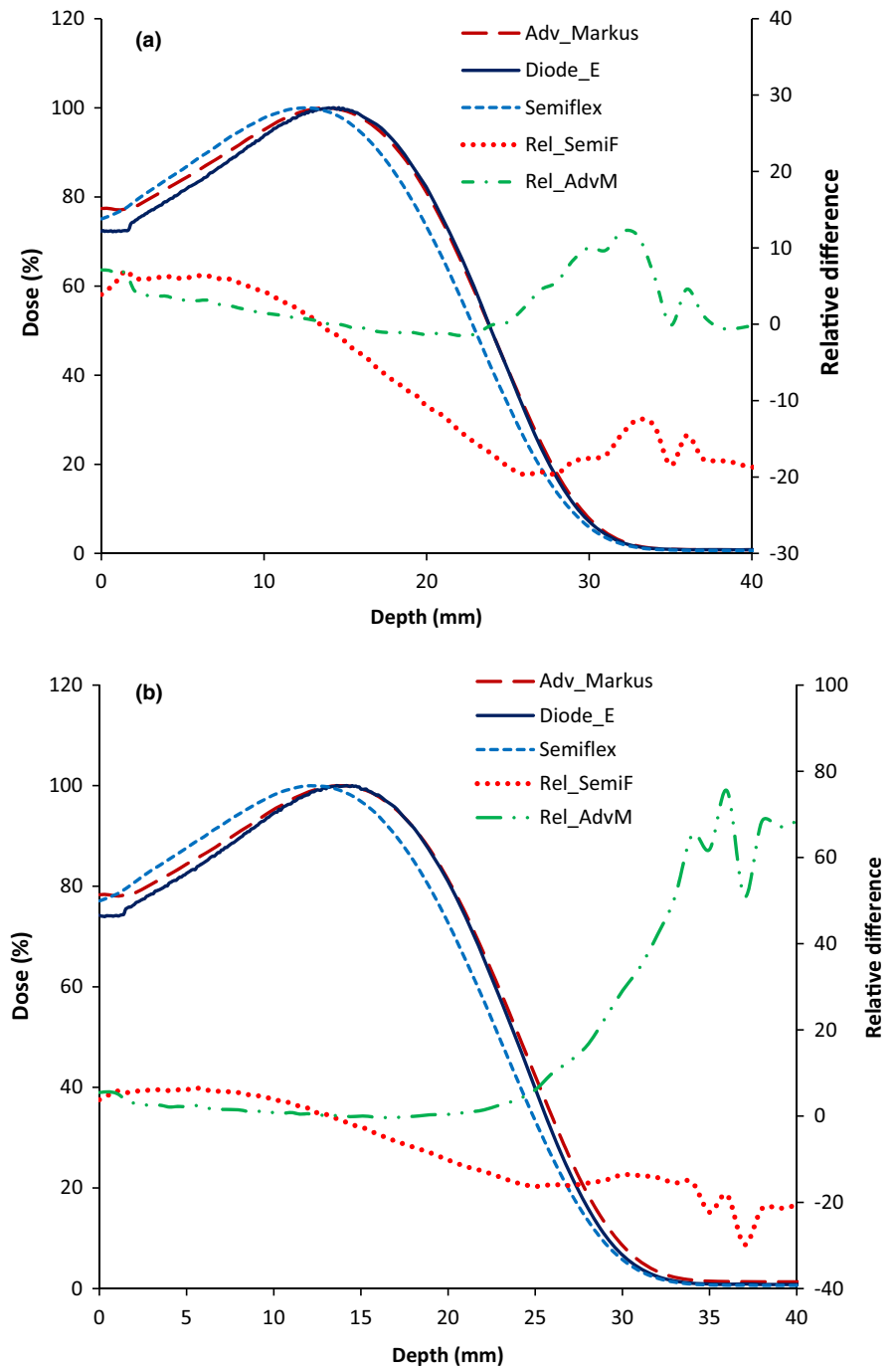
FIG. 1. Percentage depth dose (PDD) curves for a 6 MeV electron beam measured with the Semiflex, Advanced Markus, and Diode-E detectors. PDDs are for (a) 10 \times 10 \text{ cm}^2 and (b) 25 \times 25 \text{ cm}^2 electron field sizes. Relative differences with respect to the diode PDD are also shown (axis on the right side).
