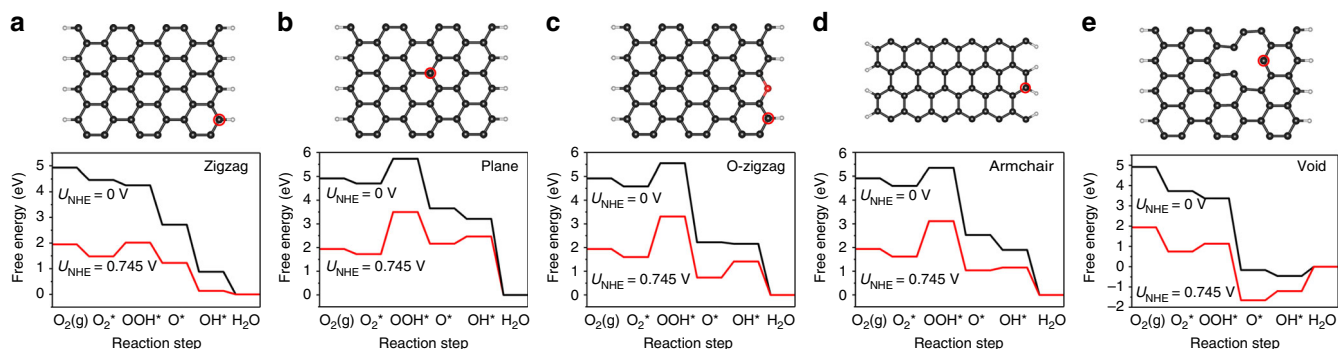
Fig. 5 Theoretical calculations. Models (top) and the corresponding free energy diagrams (bottom) for cycled carbon atoms at electrode potential U_{\text{NHE}} = 0 and 0.745 V in 0.5 M \text{H}_2\text{SO}_4 (NHE normal hydrogen electrode, RHE reversible hydrogen electrode, U_{\text{NHE}} = U_{\text{RHE}} - 0.0591 \times \text{pH} , \text{pH} = 0.25 ). a Carbon atom at zigzag edge, b carbon atom in basal plane, c carbon atom at O-doped zigzag edge, d carbon atom at armchair edge, and e carbon atom near a void
