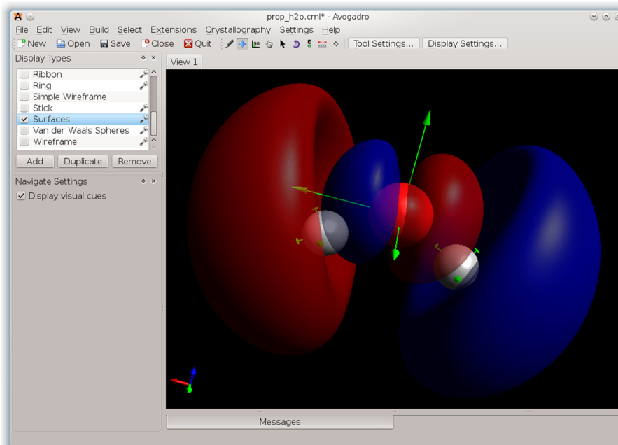
Figure 2 Visualization of molecular orbital isosurface calculated by Avogadro using the NWChem CML data, with NMR tensor projections and magnitudes represented as arrows.
