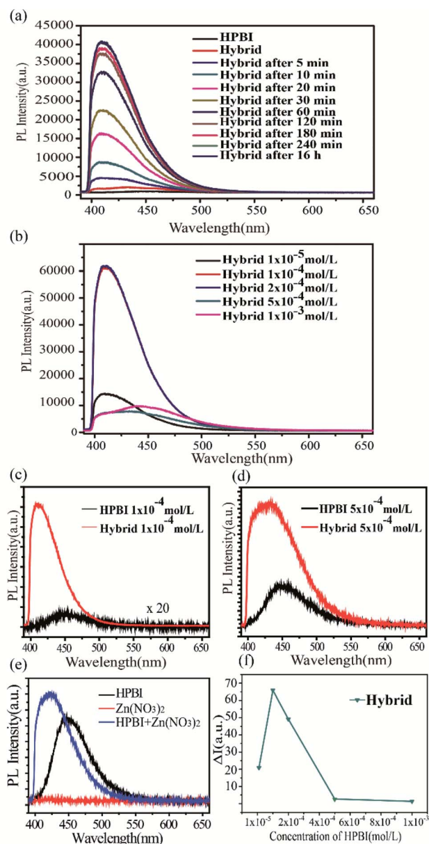
Fig. 5 (a) Fluorescence spectra of ZIF-8 with immersion time increased in the presence of HPBI ( 1 \times 10^{-4} mol L -1 ). (b) Fluorescence spectra of ZIF-8 in the presence of various concentrations of HPBI under excitation at 375 nm. (c) and (d) Comparing fluorescence spectra of HPBI and ZIF-8 (hybrid) with corresponding concentrations of HPBI ( 1 \times 10^{-4} mol L -1 and 5 \times 10^{-4} mol L -1 ), the intensity of HPBI ( 1 \times 10^{-4} mol L -1 ) multiply by 20 in order to see the peak position (black line). (e) Comparing fluorescence spectra of HPBI and HPBI + Zn(NO 3 ) 2 . (f) \Delta I denotes the enhanced fluorescence intensity of HPBI with different concentrations after adding ZIF-8.
