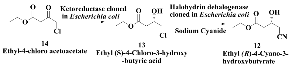
Figure 3. Atorvastatin: Enzymatic preparation of ( R )-4-cyano-3-hydroxybutyrate.
