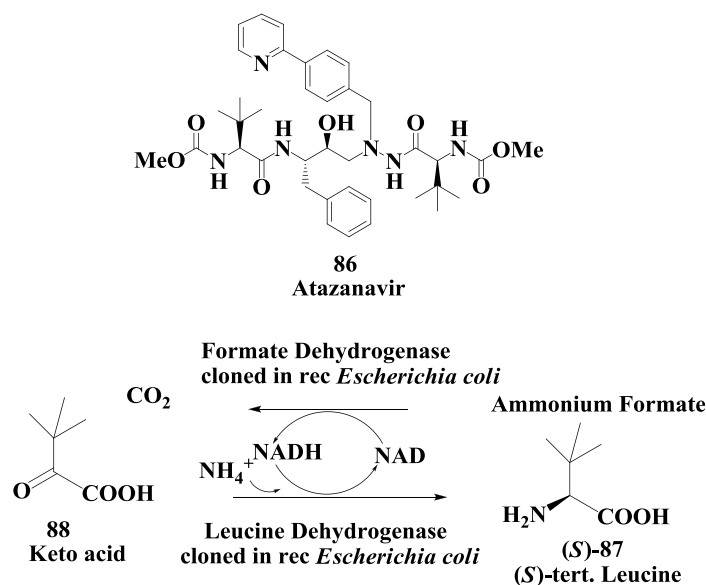
Figure 22. Atazanavir (anti-viral agent): Enzymatic synthesis of ( S )-tertiary-leucine.
