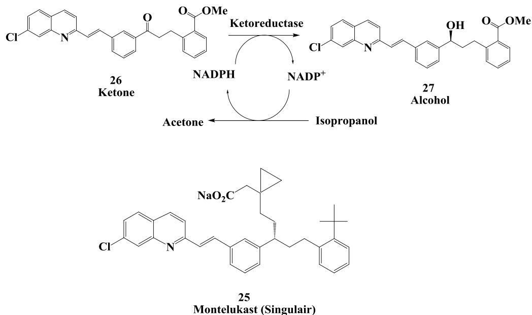
Figure 7. Enzymatic reduction process for synthesis (S)-alcohol 27 for Montelukast intermediate.
