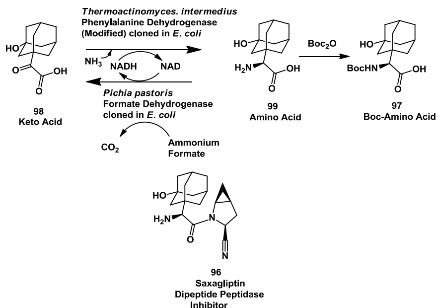
Figure 26. Saxagliptin: Enzymatic reductive amination of 2-(3-hydroxy-1-adamantyl)-2-oxoethanoic acid.
