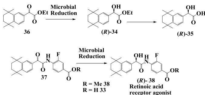
Figure 10. Retinoic acid receptor agonist: Enzymatic preparation of 2-( R )-hydroxy-2-(1',2',3',4'-tetrahydro-1',1',4',4'-tetramethyl-6'-naphthalenyl)acetate.
