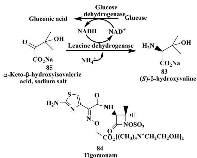
Figure 21. Tigemonam: Enzymatic synthesis of ( S )- \beta -hydroxyvaline.
