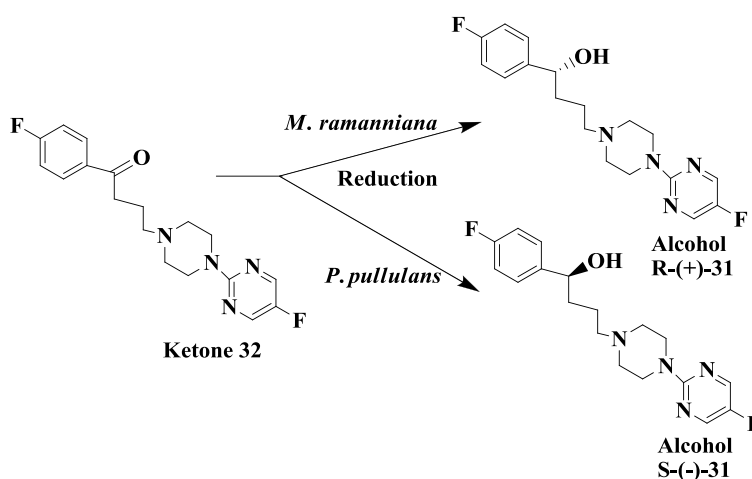
Figure 9. Antipsychotic drug: Enzymatic reduction of 1-(4-fluorophenyl)4-[4-(5-fluoro-2-pyrimidinyl)1-piperazinyl]-1-butanone.
