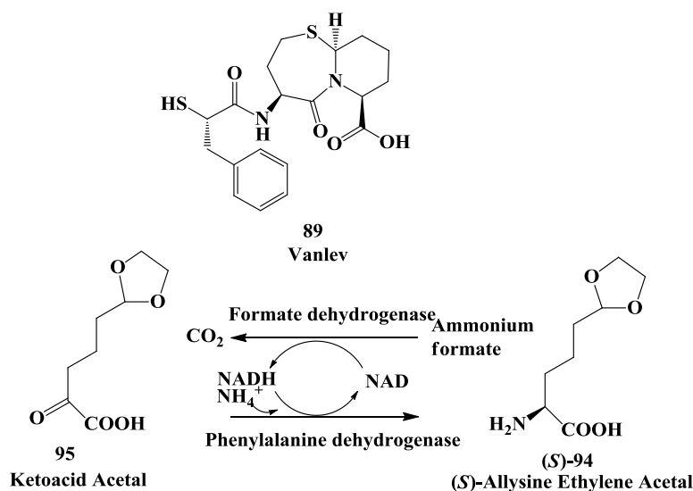
Figure 25. Vanlev: Enzymatic synthesis of allysine ethylene acetal.
