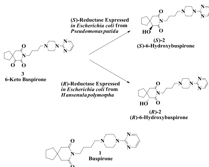
Figure 1. Hydroxy buspirone (antianxiety drug): Enzymatic preparation of 6-hydroxybuspirone.
