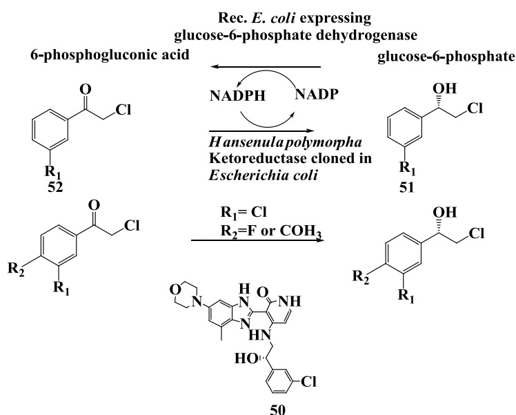
Figure 13. Anticancer drug: Enzymatic preparation of ( S )-2-chloro-1-(3-chlorophenyl)ethanol.
