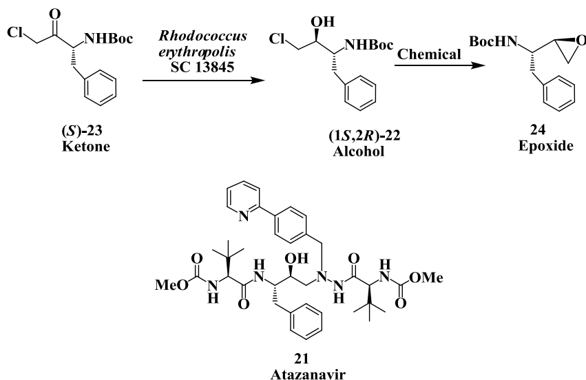
Figure 6. Atazanavir (antiviral agent): Enzymatic reduction of (1 S ,2 R )-[3-chloro-2-hydroxy-1-(phenylmethyl) propyl]-carbamic acid,1,1-dimethyl-ethyl ester.
