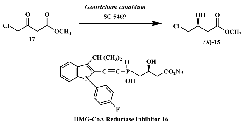
Figure 4. Cholesterol lowering agents: Preparation of ( S )-4-chloro-3-hydroxybutanoic acid methyl ester.
