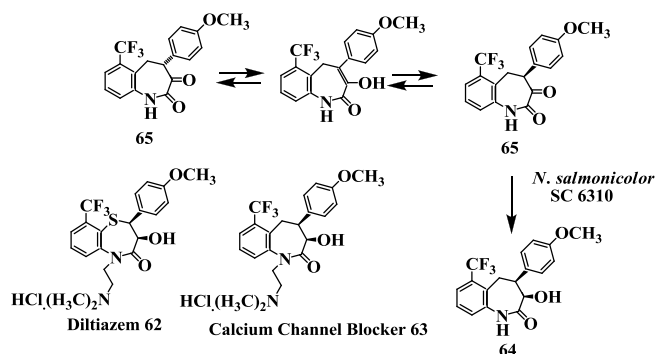
Figure 16. Calcium channel blocker: Preparation of [(3 R - cis )-1,3,4,5-tetrahydro-3-hydroxy-4-(4-methoxyphenyl)-6-(trifluoromethyl)-2 H -1-benzazepin-2-one].
