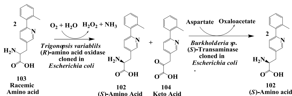
Figure 28. Glucogen like peptide: The (S)-amino-3-[3-{6-(2-methylphenyl)}pyridyl]-propionic acid.
