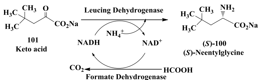
Figure 27. Enzymatic synthesis of ( S )-neopentylglycine.
