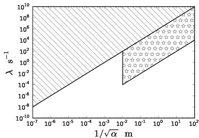
Figure 3. CSL parameter diagram. The hatched area shows the region of \lambda - \alpha parameter space currently ruled out by diffraction experiments. The starred area shows the region of parameter space in which the correlated random walks are experimentally accessible.
