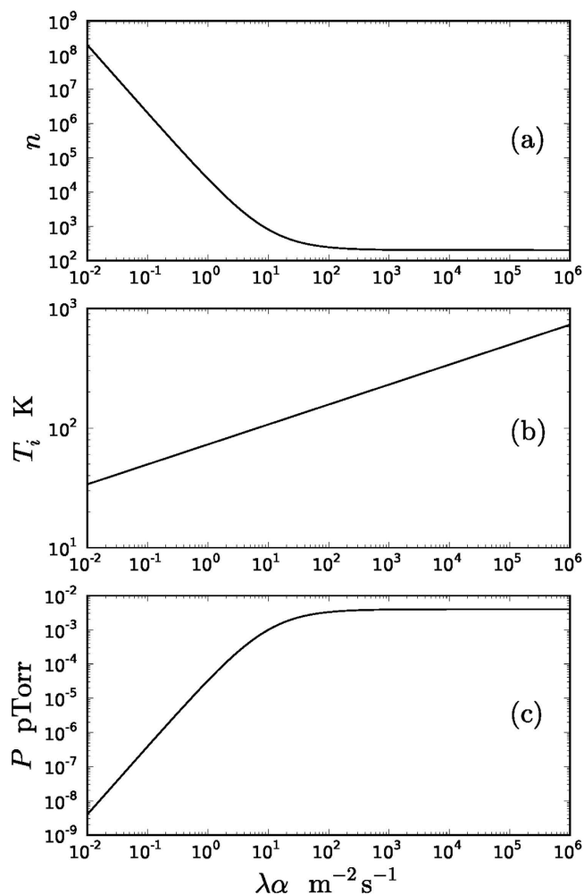
Figure 2. (a) Minimum value for the number of observations n required to estimate the variance \sigma_{CSL}^2 with sufficient accuracy. The statistical error in the estimate should be an order of magnitude less than \sigma_{CSL}^2 . (b) Maximum internal temperature T_i of particles required to prevent significant thermal diffusion by emission of radiation. (c) Maximum ambient pressure P required to prevent significant diffusion due to collisions between ambient molecules and the nanoparticles of interest. In cases (b) and (c) the boundary is determined by the requirement that the environmental contributions to the variance of the displacement of the nanoparticle should be less than \sigma_{CSL}^2 by an order of magnitude.
