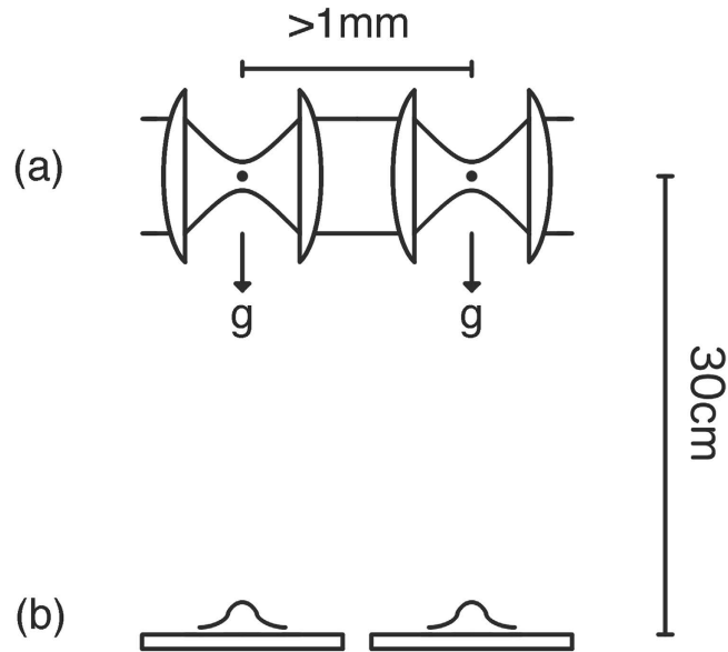
Figure 1. The experimental setup: (a) Laser light creates adjacent harmonic traps for two nanoparticles separated by of order 1mm. The particles are simultaneously released and fall 30 cm. During this period the wave packets of the two particles undergo quantum dispersion. A dynamical wavefunction collapse mechanism will also cause diffusion of the centre of mass of each of the wave packets. The diffusions of the two packets will be correlated if the localization length scale is greater than the particle separation. The position of each particle is recorded with 10 nm accuracy at (b).
