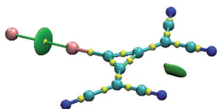
Fig. 2 Optimized geometries of the [1, \text{I}^-] complex with (3, -1) bond critical points (yellow spheres) and the bond path (green line) from the QTAIM analysis. The blue–green disc indicates intermolecular attractive interactions resulting from the NCI treatments ( s = 0.4 a.u. iso-surfaces, color scale: -0.035 (blue) < \rho < 0.02 (red) a.u.).
