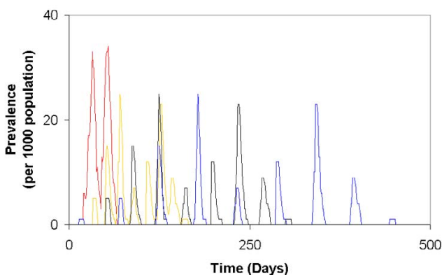
Figure 5 Prevalence of a disease (per 1000 population) based on different values of \omega_i . Here, \omega_i = 1.0 \times 10^{-1} (red curve), 1.0 \times 10^{-3} (yellow curves), 1.0 \times 10^{-6} (black curves), and 1.0 \times 10^{-9} (blue curves).
