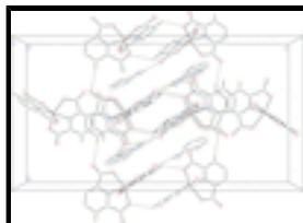
Fig. 2. Packing of I viewed down a with H-bonding interactions shown as dashed lines. Displacement ellipsoids are drawn at the 30% probability level. H atoms not involved in hydrogen bonding are omitted. Key: Fe = brown, O = red, N = blue, C = grey, H = green.
