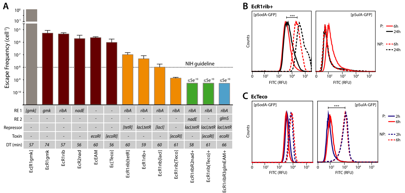
Figure 3. Layering of multiple safeguards reduces escape. (A) Escape frequencies ( n = 3 , \pm SD) on solid media for strains containing one (red), two (orange), three (green) or four (blue) layers of genetic safeguards. NIH guidelines for work with engineered microorganisms advise a 10^{-8} escape frequency (11) (dotted horizontal line). Strains are characterized by ribo-essential gene (RE 1 or 2), presence of supplemental repressors, presence of a toxin and doubling time (DT) in minutes. Plasmid-based ribo-essential gmk safeguard (gray) does not confer containment. Square brackets denote plasmid-based constructs. Limit of detection for solid media is \sim 5 \times 10^{-10} . Flow cytometry shows fluorescence from sodA and sulA promoters in EcR1rib+ (B) or EcTeco (C) when grown in non-permissive media (dashed) versus permissive (solid) media for 2 (purple), 6 (red) or 24 (black) h. *** denotes P \leq 0.001 , Student's one-tailed t -test with Welch's correction.
