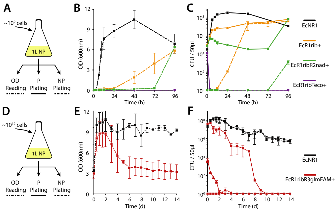
Figure 4. Large volume and long-term challenge of multilayered safeguard strains. (A) Strains grown in permissive (P) media to \sim 10^9 cells then challenged over 96 h in 1 l of non-permissive (NP) media, which is monitored for cell density (OD) (B) and cell viability (CFU) on permissive (solid line) and non-permissive (dotted line) solid plates (C). Biological triplicate results for control strain (EcNR1, black), 2-layer strain (EcR1rib+, orange), 3-layer strain (EcR1ribR2nad+, green) and 3-layer bacteriotoxic strain (EcR1rib[Teco]+, purple) plotted. (D) Control (EcNR1, black) and 4-layer safeguard (EcR1ribR3glmEAM+, red) strains grown in permissive, then challenged in 1 l of non-permissive media. (E) Strains were monitored by OD readings (F) and by plating on permissive or non-permissive solid media over 14 days (squares, \sim 10^{12} cell inoculum) or 5 days (triangles, \sim 10^8 cell inoculum). No colonies were observed on NP media for the 4-layer strain.
