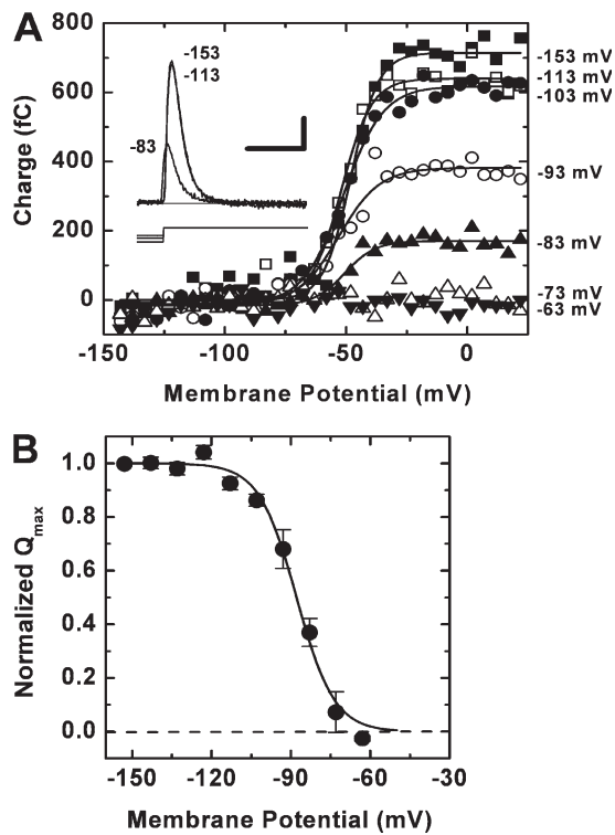
Figure 3. Holding potential dependence of Q availability. (A) Q_{ONV} curves were generated between -143 and +22 mV in 5 -mV increments from the indicated holding potentials, and the start-to-start interval was 7 s. Each curve was described by assuming a Boltzmann function to estimate the maximal Q ( Q_{ON-MAX} ). Inset, gating currents were elicited by step depolarizations to +2 mV from the indicated holding potentials. The scale bars correspond to 5 ms and 500 pA. (B) The holding potential dependence of normalized Q_{ON-MAX} was described by assuming a Boltzmann function with the following best-fit parameters: V_{1/2} = -88 mV and z = 3.6 e_0 ; n = 3-7 independent determinations.
