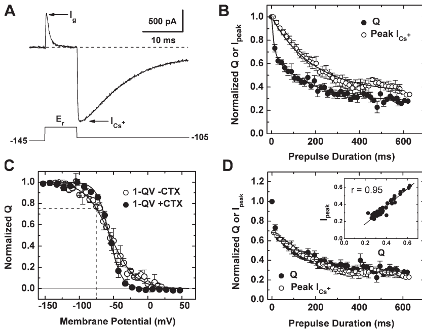
Figure 8. Simultaneous measurements of inactivation and Q-immobilization. (A) Simultaneous measurement of gating and ionic currents was accomplished by a step depolarization to the \text{Cs}^+ reversal potential ( E_r = +35 mV; Materials and methods) to isolate the gating current and a subsequent hyperpolarization to -105 mV to evoke a \text{Cs}^+ tail current. Gating charge immobilization was assayed as the fraction of total charge remaining after a prepulse of variable duration to -75 mV, while inactivation was assayed by the fraction of tail current remaining in the same trace. The dashed line indicates the zero current level. (B) Gating charge immobilization (filled circles) was described assuming a bi-exponential function with the following best-fit parameters: \tau_{\text{fast}} = 10.8 ms, relative weight = 0.31; \tau_{\text{slow}} = 190 ms, relative weight = 0.43; and the relative weight of nonimmobilized Q = 0.25 . Inactivation (hollow circles) was described by assuming an exponential function with the following best-fit parameters: \tau = 228 ms, relative weight = 0.75; relative weight of noninactivated current = 0.25. The fast phase
