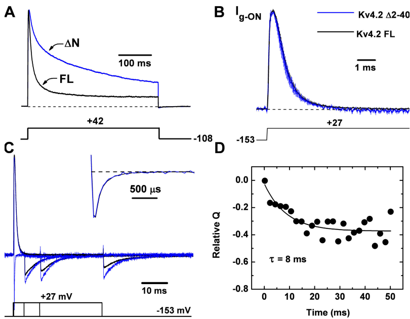
Figure 10. The Kv4.2 N terminus slows Q_{\text{OFF}} at depolarized potentials. (A) Ionic currents were elicited by a voltage step from -108 mV to +42 mV for full-length Kv4.2 (FL, black line) and \Delta 2-40 Kv4.2 ( \Delta N , blue line) channels. (B) I_{g\text{ON}} was elicited by a voltage step from -153 to +27 mV. Current traces represent the average of five (Kv4.2) and three ( \Delta 2-40 Kv4.2) experiments and the vertical lines correspond to the standard errors. (C) Average I_{g\text{S}} were normalized to the I_{g\text{ON}} to compare the I_{g\text{OFF}} s measured by hyperpolarizations to -153 mV after depolarizations of increasing duration to +27 mV. To determine the contribution of the N terminus to Q -immobilization in a curve-fitting independent manner, the relative Q difference was measured by integrating the area bounded by the two I_{g\text{OFF}} current traces from Kv4.2 and \Delta 2-40 Kv4.2 channels. Inset, overlay I_{g\text{OFF}} s after a 0.2-ms depolarization. (D) An exponential function with \tau corresponding to the fast time constant of macroscopic inactivation of Kv4.2 channels (8 ms) adequately described the increase in the relative Q difference over time (solid line).
