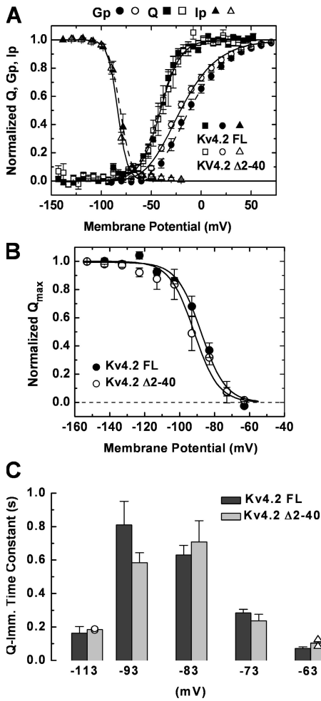
Figure 11. Steady-state Q-immobilization is independent of the Kv4.2 N terminus. (A) Gp-V (circles), Q_{ON}V (squares), and I_{SS} (triangles) curves from Kv4.2 (black symbols) and \Delta 2-40 Kv4.2 (hollow symbols) channels were analyzed as described under Materials and methods (Data Analysis). The best-fit parameters were as follows: Gp-V V_{1/2} = -13 mV (Kv4.2), -22.2 mV ( \Delta 2-40 Kv4.2), k = 23.2 mV (Kv4.2), k = 23.2 mV ( \Delta 2-40 Kv4.2); Q_{ON}V V_{1/2} = -42 mV (Kv4.2), -43 mV ( \Delta 2-40 Kv4.2), z = 2.4 e_0 (Kv4.2), z = 2.4 e_0 ( \Delta 2-40 Kv4.2); I_{SS} V_{1/2} = -81 mV (Kv4.2), -84 mV ( \Delta 2-40 Kv4.2), k = 5.7 mV (Kv4.2), 4.9 mV ( \Delta 2-40 Kv4.2). (B) Q-availability curves from Kv4.2 (filled circles) and \Delta 2-40 Kv4.2 (hollow circles) channels were analyzed as described in Fig. 3 legend; and the best-fit parameters were as follows: V_{1/2} (Kv4.2) = -88 mV and z (Kv4.2) = 3.6 e_0 ; V_{1/2} ( \Delta 2-40 Kv4.2) = -92 mV and z ( \Delta 2-40 Kv4.2) = 3.6 e_0 ; n = 3-5 independent experiments. (C) Time constants of Q-immobilization for Kv4.2 and \Delta 2-40 Kv4.2 channels are represented as bars. Differences were not statistically significant ( P < 0.05 ). Time constants from voltages with n < 3 are represented as individual data points.
