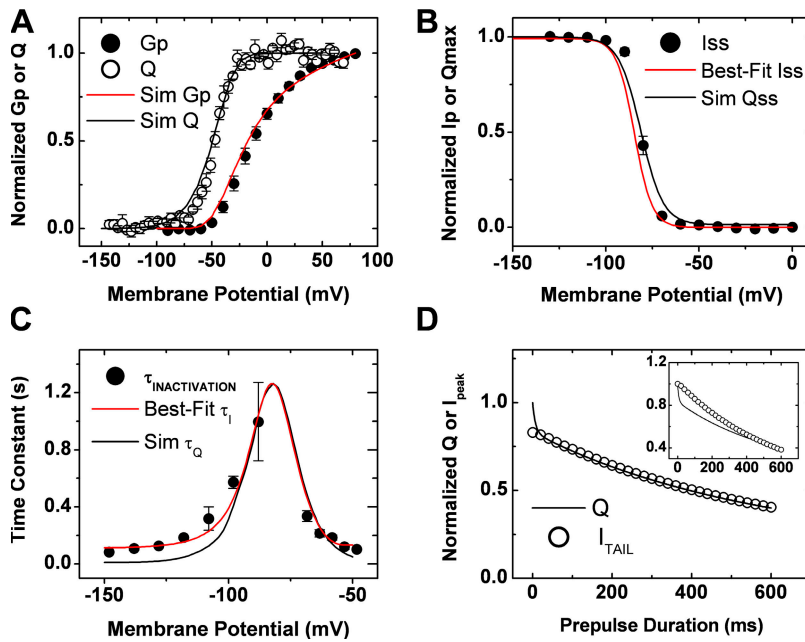
Figure 14. The ZHA + I model predicts equivalent kinetics and voltage dependence of inactivation and Q-immobilization. (A) The global best fit of the ZHA + I model ( Q_{\text{ON}}V curve, black line; Gp-V curve, red line) accurately simulates the experimental Q_{\text{ON}}V (hollow circles) and Gp-V relations (filled circles). (B) Best-fit and experimental I_{\text{SS}} (red line and filled circles, respectively) curves. The simulated Q-availability curve (Sim Q_{\text{SS}} ) is shown for comparison (black line). (C) The ZHA + I model accurately describes (best fit, red line) the voltage dependence of the time constants of inactivation (experimental data, filled circles). The simulated time constants of Q-immobilization (Sim \tau_Q ) are shown for comparison (black line). (D) Simulation of simultaneous inactivation (hollow circles) and Q-immobilization (black line) at -70 mV. Curves are renormalized as explained previously (Figs. 8 and 9). Inset, Q decay is biphasic (see text).
