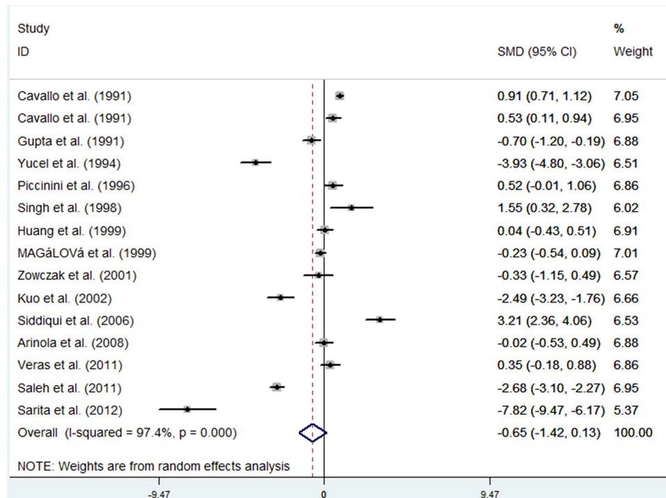
Figure 2. Forest plot showing the meta-analysis outcome of the serum zinc levels for breast cancer patients versus healthy controls.
