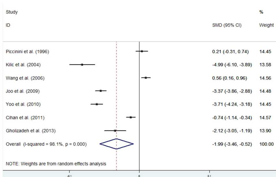
Figure 5. Forest plot showing the meta-analysis outcome of the hair zinc levels for breast cancer patients versus healthy controls.
