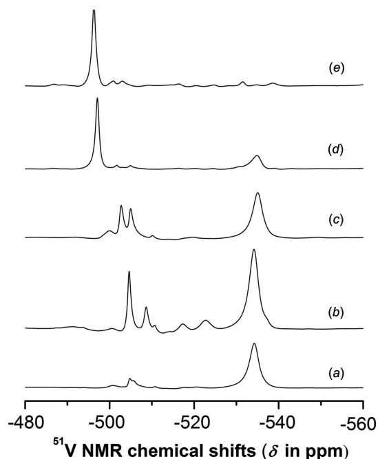
Figure 6 ( a )/( b ) The 51 V NMR spectra of the crystallization solution of VMo 7 and ( c )/( d )/( e ) solutions obtained upon dissolution of crystallized VMo 7 at different pH values. Conditions: ( a ) 175 mM Mo VI , 25 mM V V , pH = 3.1, 24 h after the synthesis; ( b ) same conditions as ( a ) after another 24 h; ( c )/( d )/( e ) 10 mM V V solution prepared from VMo 7 by dissolving it in 0.5 mM NaCl at pH values of ( c ) 4.0, ( d ) 5.2 and ( e ) 6.0. The pH was adjusted by the addition of a dilute KOH solution.
