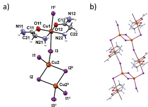
Fig. 4 (a) Molecular structure of 3c with atom labelling scheme. Cu(II) are coordinated octahedrally in the cis -HL fashion. Two Cu(I) ions, Cu2 and Cu2 ii are both coordinated tetrahedrally with a shared edge. Symmetry operators i = -x, y - 1, -z ; ii = x + 1, y - 1, z - 1 . (b) double chain of the coordination polymer.
