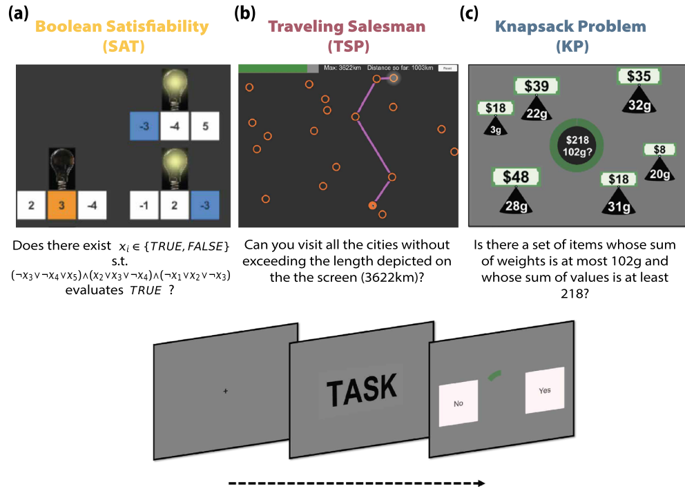
Figure 5. Experimental tasks. (a) Boolean satisfiability. In this task, the aim is to determine whether a Boolean formula is satisfiable . The Boolean formula is represented by a set of light bulbs (clauses), each of which has three switches (literals) underneath that are characterized by a positive or negative number. The number on each switch represents the variable number, which can be turned on or off (TRUE or FALSE). The aim of the task is to determine whether there exists a way of turning on and off variables such that all the light bulbs are turned on (the corresponding Boolean formula evaluates to TRUE). The task was interactive. Participants could click on switches to turn them on and the corresponding literals and light bulbs would change color automatically. This stage had a time limit of 110 s. Afterwards, participants had 3 s to make their response (either ‘YES’ or ‘NO’). (b) Traveling salesperson. Participants are given a list of cities displayed on a rectangular map on the screen and a limit L on path length. The problem is to determine whether there exists a path connecting all N cities with a distance at most L . The task was interactive. Participants could click from city to city and the corresponding path and distance traveled would display and update automatically. This stage lasted a maximum of 40 s. Afterwards, participants had 3 s to make their response. (c) Knapsack. Participants are presented with a set of items with different values and weights. Additionally, a capacity constraint and target profit are shown at the center of the screen. The aim is to ascertain whether there exists a subset of items for which (1) the sum of weights is lower or equal to the capacity constraint and (2) the sum of values yields at least the target profit. The task was not interactive. This stage lasted for 25 s. Finally, participants had 2 s to make their response.
