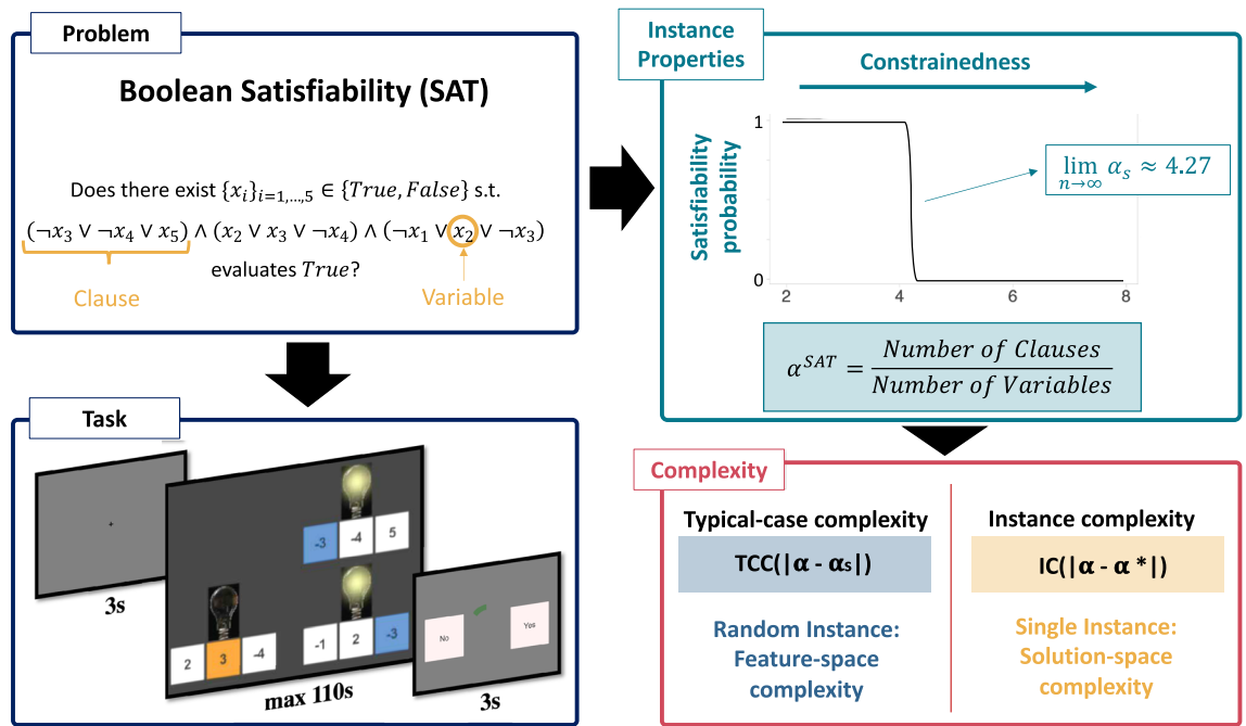
Figure 1. 3SAT problem, complexity metrics and experimental design. The problem. The aim is to determine whether a Boolean formula is satisfiable . The task. The Boolean formula is represented with a set of light bulbs (clauses), each of which has three switches underneath (literals) that are characterized by a positive or negative number. The number on each switch represents the variable number, which can be turned on or off (TRUE or FALSE). The aim is to determine whether there exists a way of turning on and off variables such that all the light bulbs are turned on (formula evaluates TRUE). Instance properties. The constrainedness of the problem ( \alpha ) is captured by the ratio of clauses to variables. This parameter characterizes the probability that a random instance of the problem is satisfiable. In the limit this probability undergoes a phase transition around the satisfiability threshold ( \alpha_s ). Complexity metrics. Instances near this threshold are on average harder to solve than instances further away. Average hardness is captured by typical-case complexity (TCC). This metric can be estimated entirely from the features of the problem (feature-space) without the need to solve the problem. Alternatively, instance complexity (IC) can be estimated from features of the solution-space. IC is defined as the difference between the constrainedness of the instance ( \alpha ) and \alpha^* , the maximum number of clauses that can be satisfied divided by the number of variables in the instance.
