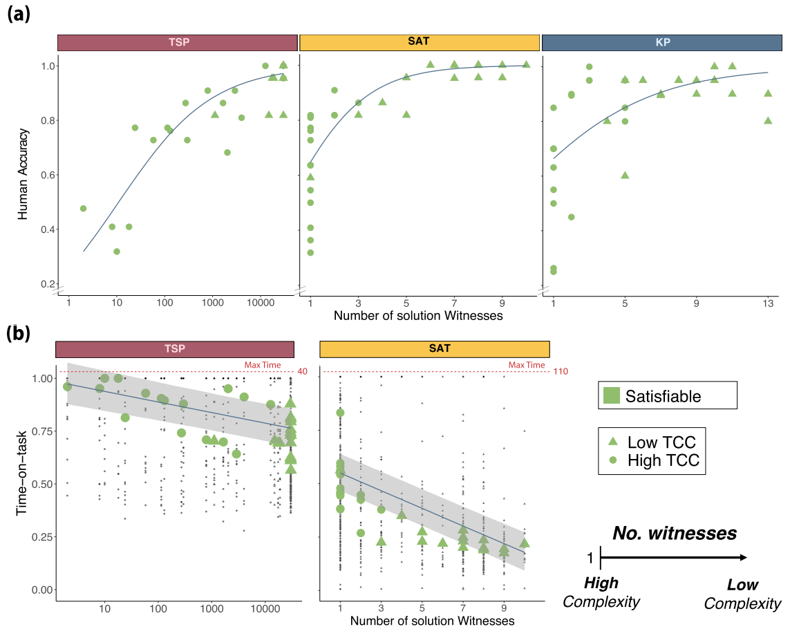
Figure 3. Number of solution witnesses. The number of witnesses is defined as the number of state-space combinations (i.e., paths, selection of items or switch-setups) that satisfy the constraints. On satisfiable instances, the problem becomes harder as the number of witnesses approaches 1. Only satisfiable instances are included. (a) Human accuracy. Each green shape represents the mean accuracy per instance. The blue line represents the marginal effect of the number of solution witnesses on human accuracy (GLMM Supplementary Table S5 Models 1,4,7). (b) Time-on-task. Each green shape represents the median time-on-task per instance. The blue line represents the marginal effect (and 95% credible interval) of the number of solution witnesses on time-on-task (CLMM Supplementary Table S3 Model 5 and Supplementary Table S4 Model 5). Each black dot corresponds to the time-on-task of one participant while solving a single instance.
