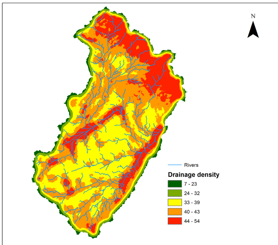
Figure 8. The drainage density map of the Makutupora basin.
