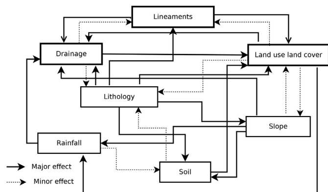
Figure 3. Dependency of factors influencing groundwater recharge.
