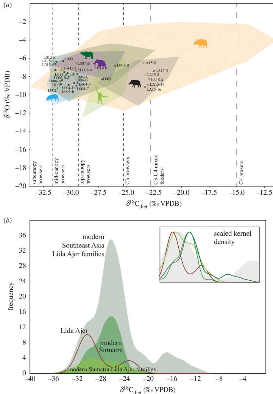
Figure 3. Stable isotope analysis of \delta^{13}\text{C}_{\text{diet}} (‰ VPDB) and \delta^{18}\text{O} (‰ VPDB) from faunal enamel of mammals from Lida Ajjer. (a) Comparison of Lida Ajjer specimens (closed circles indicate fossils sampled directly from Lida Ajjer; open circles represent fossils sampled from the Naturalis) against all Southeast Asian representatives from those families (convex hulls). Divisions between canopy browsers indicative and based on Louys & Roberts [25]. Animal silhouettes from Phylopic.org (public domain and CC BY-SA 3.0 CC BY 3.0 Pongo by Gareth Monger and CC BY-NC 3.0 Elephantini by Zimices). (b) Kernel density plots for Lida Ajjer and modern subsets of Southeast Asian mammals. Inset: kernel densities artificially scaled to the same frequency and compared against a subtropical monsoon forest in China; drawn after Tejada et al. [31] using data from Ehleringer et al. [32]. (Online version in colour.)
