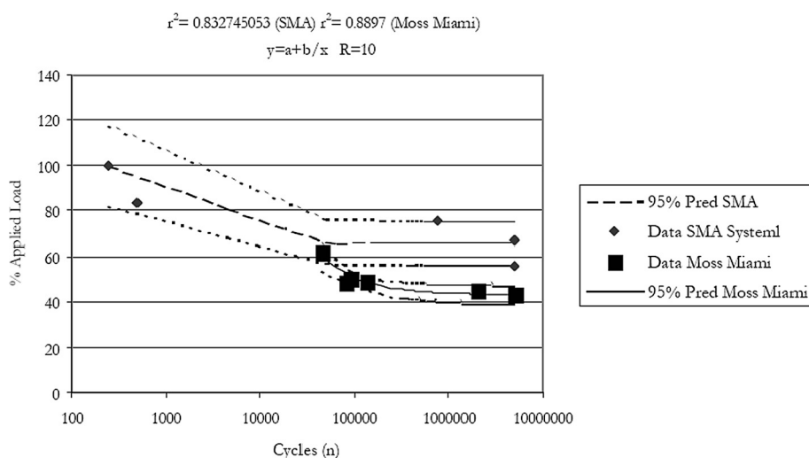
Figure 5 Axial compression bending fatigue curves for the memory metal spinal system (sma) & the moss Miami system.
