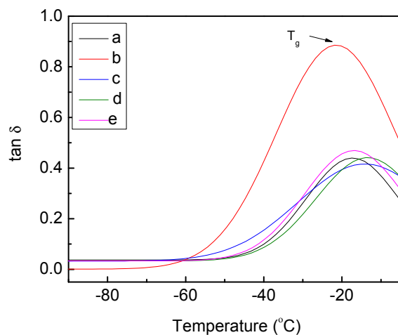
Figure 10. Temperature dependence of the \tan\delta of polyurethane (a) unmodified; and loaded with (b) 10% (w/w) AgNO 3 ; (c) 1% (w/w) Ag lactate; (d) 10% (w/w) Ag lactate; and (e) Ag nanoparticles.
