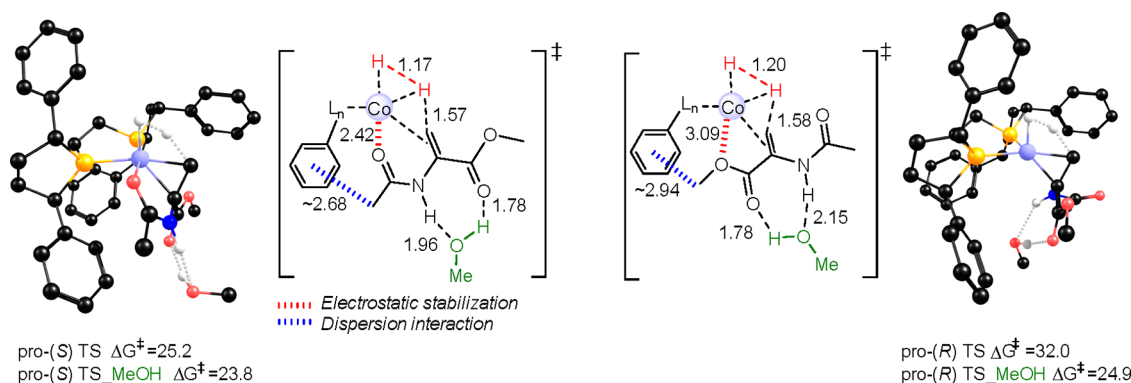
Figure 6. Optimized pro -( S ) (left) and pro -( R ) (right) hydride transfer TSs for (R,R) - (\text{Ph})\text{BPECo} -catalyzed hydrogenation of MAA via redox mechanism A, with a hydrogen-bonded MeOH molecule (barriers relative to \text{Co}(0)\text{-Sub} with or without MeOH, respectively, in kcal/mol, 323 K, distances in angstroms). Hydrogens bonded to carbon are omitted for clarity. Electrostatic and dispersion interactions that favor the ( S )-TS are indicated.
