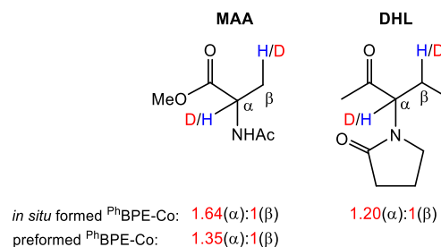
Figure 2. HD partitioning results for DHL and MAA (see Experimental Details).
