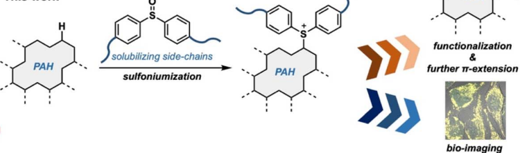
Fig. 1 Current strategies for PAH solubilization and regioselective arene functionalization. (A) Dissolution of PAHs. (B) Regioselective sulfoniumization of small arenes via thianthreneation. (C) This work.
