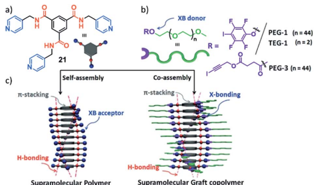
Fig. 12 (a and b) Molecular structure of BTA 21 (a) and the halogen bonding donors (b) used for orthogonal secondary binding for graftable supramolecular (co)polymers. (c) Schematic representation of the self-assembly of 21 in the absence (left) and presence (right) of orthogonal halogen bonding donors. Adapted with permission from ref. 121. Copyright 2020 Royal Society of Chemistry.
