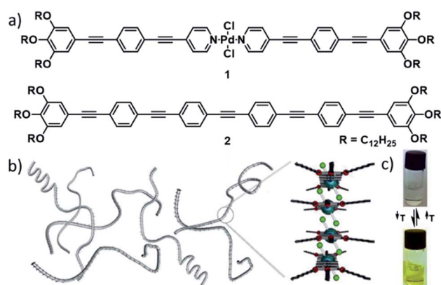
Fig. 2 (a) Molecular structures of Pd^{II} complex 1 and reference OPE 2 . (b) Schematic depiction of self-assembled fibres of 1 and the molecular packing around the metal centre. (c) Photographs of solutions of 1 showing the color change upon reversible self-assembly through temperature variation. Panels (b) and (c) adapted with permission from ref. 53. Copyright 2013 American Chemical Society.
