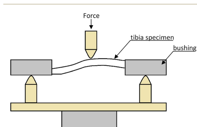
Fig. 1 Measuring setup for three-point bending of tibiae.
