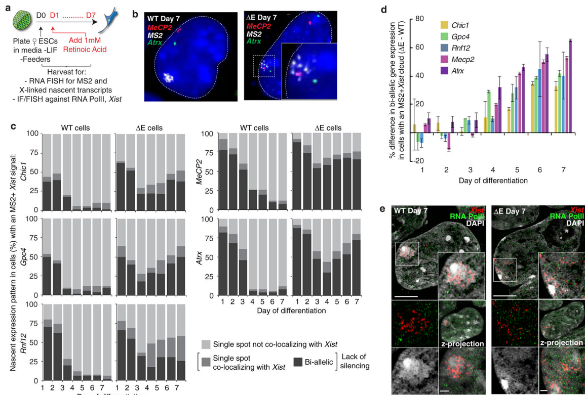
Fig. 2: The E-repeat establishes heritable gene silencing
