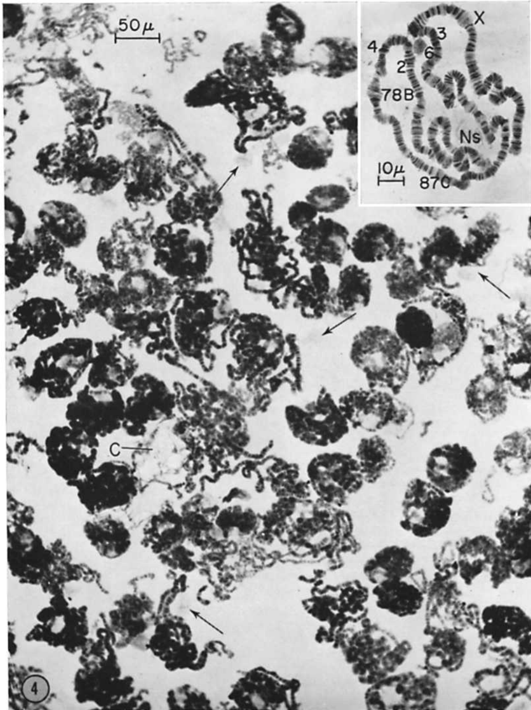
FIGURE 4 Isolated nuclei, gently squashed after orcein staining. Cytoplasmic contamination is indicated by C. Nucleoli, which are easily separated from the chromosomes by squashing, are designated by arrows. Insert, salivary gland chromosomes of an isolated nucleus obtained from late third instar larvae. The locations of the nucleolus ( Ns ) and some of the prepupal chromosome puffs are indicated. Chromosome numbers are given according to Berendes (14). \times 220 . Insert, \times 600 .
