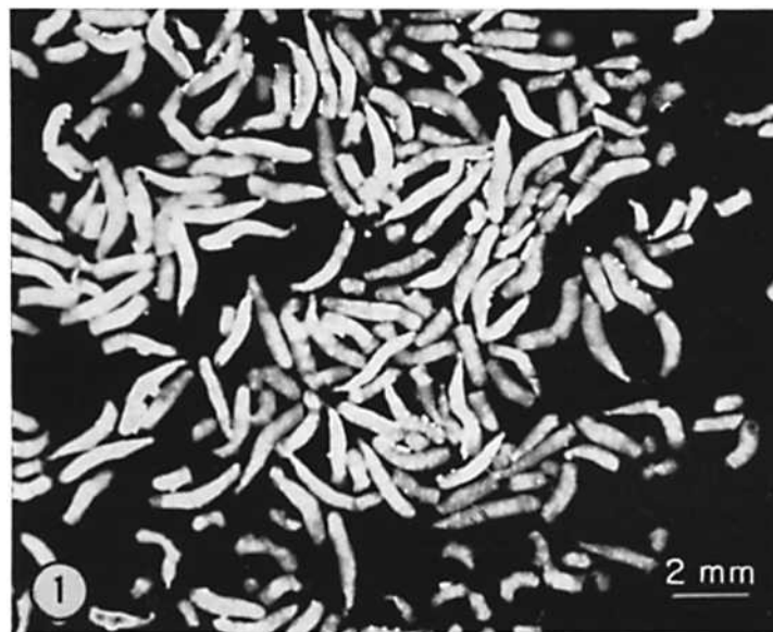
FIGURE 1 Mass-isolated salivary glands. Polaroid photograph. Glands were isolated from late third instar larvae weighing an average of 4.6 mg each. The smaller pieces are fragments of salivary glands. The white material seen attached to some glands is fat body. \times 5 .
