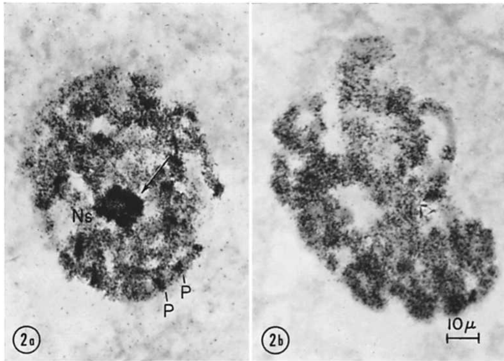
FIGURE 2 Labeling patterns of mass-isolated salivary glands. a , Tritiated-uridine incorporation into the nucleus. Specific labeling is found in the chromosome puffs ( P ) and in the nucleolus ( Ns ). b , Tritiated-thymidine incorporation into the nucleus. Discontinuous labeling can be seen in the spread chromosome on the right. \times 800 .
