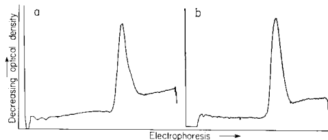
FIG. 3 Deoxyribonuclease activity in hand- and mass-prepared salivary glands. Enzyme activity was detected in acrylamide gel after disc electrophoresis according to Boyd and Mitchell (13). Gels containing native DNA were incubated for 2 hr at pH 4 in the presence of EDTA. a , Hand-Prepared glands; b , Ficoll-prepared glands.
