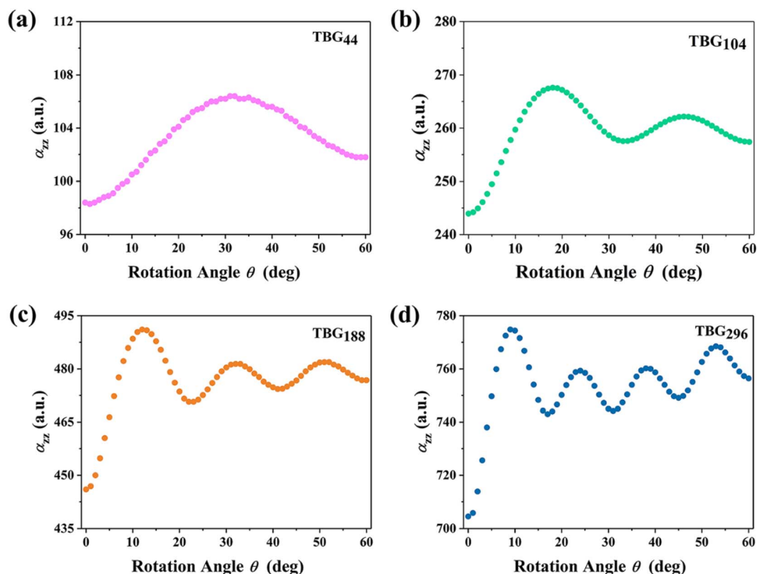
Fig. 3 (a–d) The axial polarizability ( \alpha_{zz} ) of the constructed TBG QDs varies as a function of twist angle ( \theta ).
