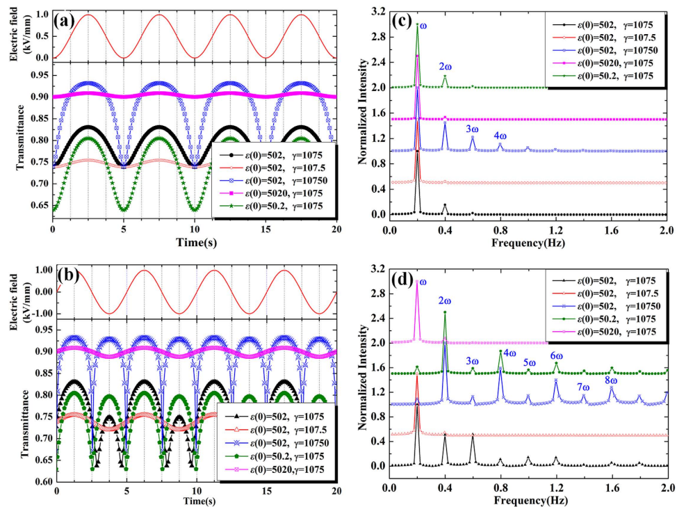
Figure 5. (a,c) are the simulations calculated from equation (5) under the electric field wave of E = E_0(\sin(\omega t) + 1) ( E = 0.5 kV/mm) and the corresponding FFTs, respectively. (b,d) are the simulations calculated from equation (5) under the electric field wave of E = E_0\sin(\omega t) ( E = 1.0 kV/mm) and the corresponding FFTs, respectively. The main harmonic signals have been labeled in frequency domain.
