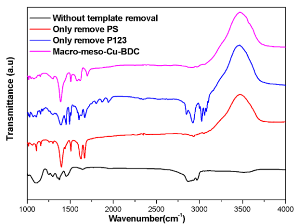
Figure S4. FT-IR spectra of macro-meso-Cu-BDC, the sample without template removal, the sample only remove of PS and the sample only remove of P123, respectively. (related to Figure 3)
