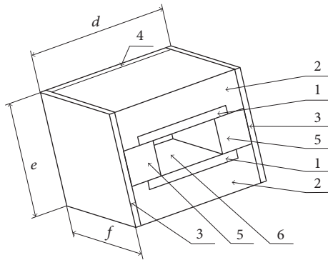
FIGURE 1: Cell culture chambers: chamber A, dimensions: d = 98 mm, e = 80 mm, f = 104 mm; chamber B, dimensions: d = 98 mm, e = 110 mm, f = 104 mm.
