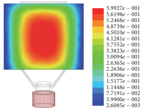
FIGURE 2: Magnetic flux distribution (flux density in T) in one of the test chambers, permanent magnets dimensions: 66 \times 11 \times 72 mm.
