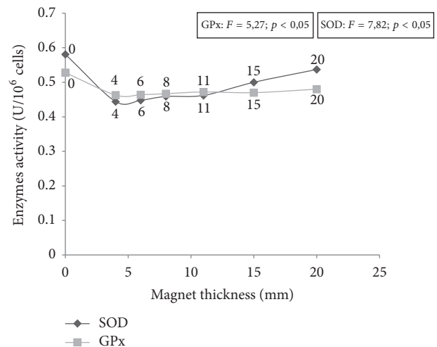
FIGURE 4: Effect of the static magnetic field on antioxidant enzymes (SOD and GPx) activity determined in fibroblasts cultures exposed to action of magnets with various thickness (4–20 mm) and control fibroblasts culture not exposed to magnet's action, with statistical evaluation ( F , p —the values of ANOVA test).
