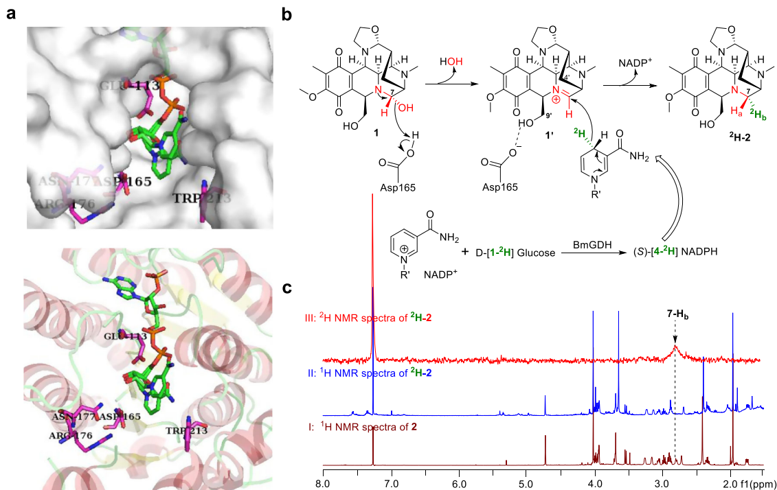
Fig. 3 Enzymology characterization of NapW-catalyzed reduction in NDM biosynthesis. a Crystal structure of NapW-NADP + complex. In this cartoon model, polar amino acids (Glu113, Asp165, Arg176, Asn177, and Trp213) around nicotinamide terminal shown as sticks. b Proposed enzymatic mechanism. c NMR analysis of enzymatic products.
