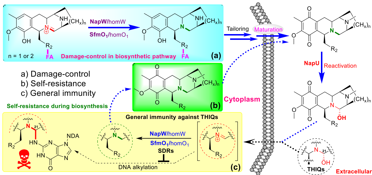
Fig. 7 Summary of the multi-level resistance model involved in NDM and SFM biosynthesis. a Damage-control process in secondary metabolic pathway controls the efficiency of biosynthetic machinery. b Self-resistance during biosynthesis by NapW-homologs ensures the safety of antibiotic-producing strains. c General immunity against THIQs is not only involved in antibiotic-producing hosts, but also exists in non-antibiotic-producing microbes containing NapW-homologs.
