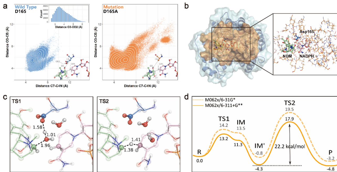
Fig. 4 The MD simulations and QM/MM calculations for NapW/NADPH-NDM model. a The two-dimensional scatter plot of distance C7-C4N and O3-CB. The wild-type system was shown in blue and the mutation system was shown in orange. In each model subplot, the structure of active site including NDM (green), NADPH (pink), and residue 165 (blue or orange) was shown in the bottom right. The important atoms and distances were annotated in gray. The distance O3-OD2 was counted and shown in the wild in the upper right in the wild-type system subplot. b The computational model for QM/MM calculations. The protein NapW was shown in blue while the orange part was represented the computational model. The QM region was shown in the form of a ball and stick model on the right. The part shown in the line form was set in MM region. c The optimized structures of key transition states (TSs). The key distances related to the catalytic reaction of NapW were labeled. d The reaction energy profile for NapW/NADPH-NDM model.
