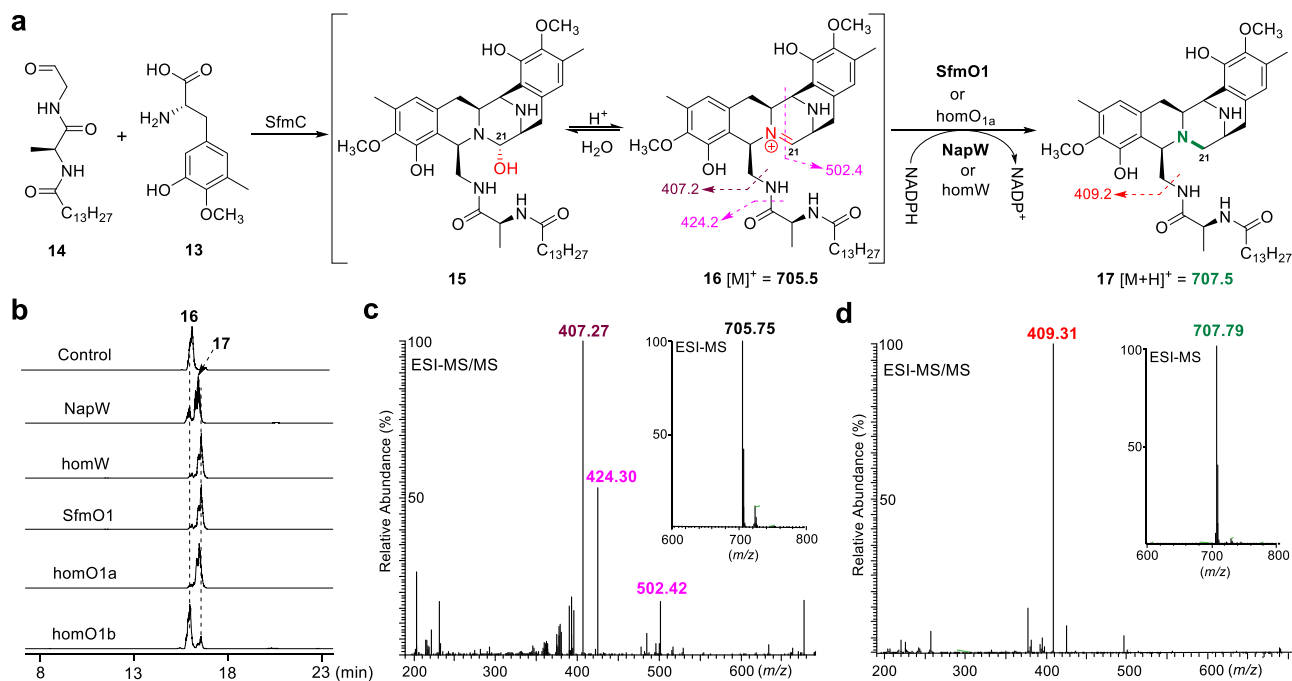
Fig. 5 Biochemical investigation of SDRs-catalyzed pharmacophore reductive quenching in SFM biosynthesis. a Enzymatic reactions mediated by SfmC and SDRs. b LC-MS analysis of enzymatic reaction products. c ESI-MS and ESI-MS/MS analysis of 16 generated by SfmC. d ESI-MS and ESI-MS/MS analysis of 17 generated by SDRs.
