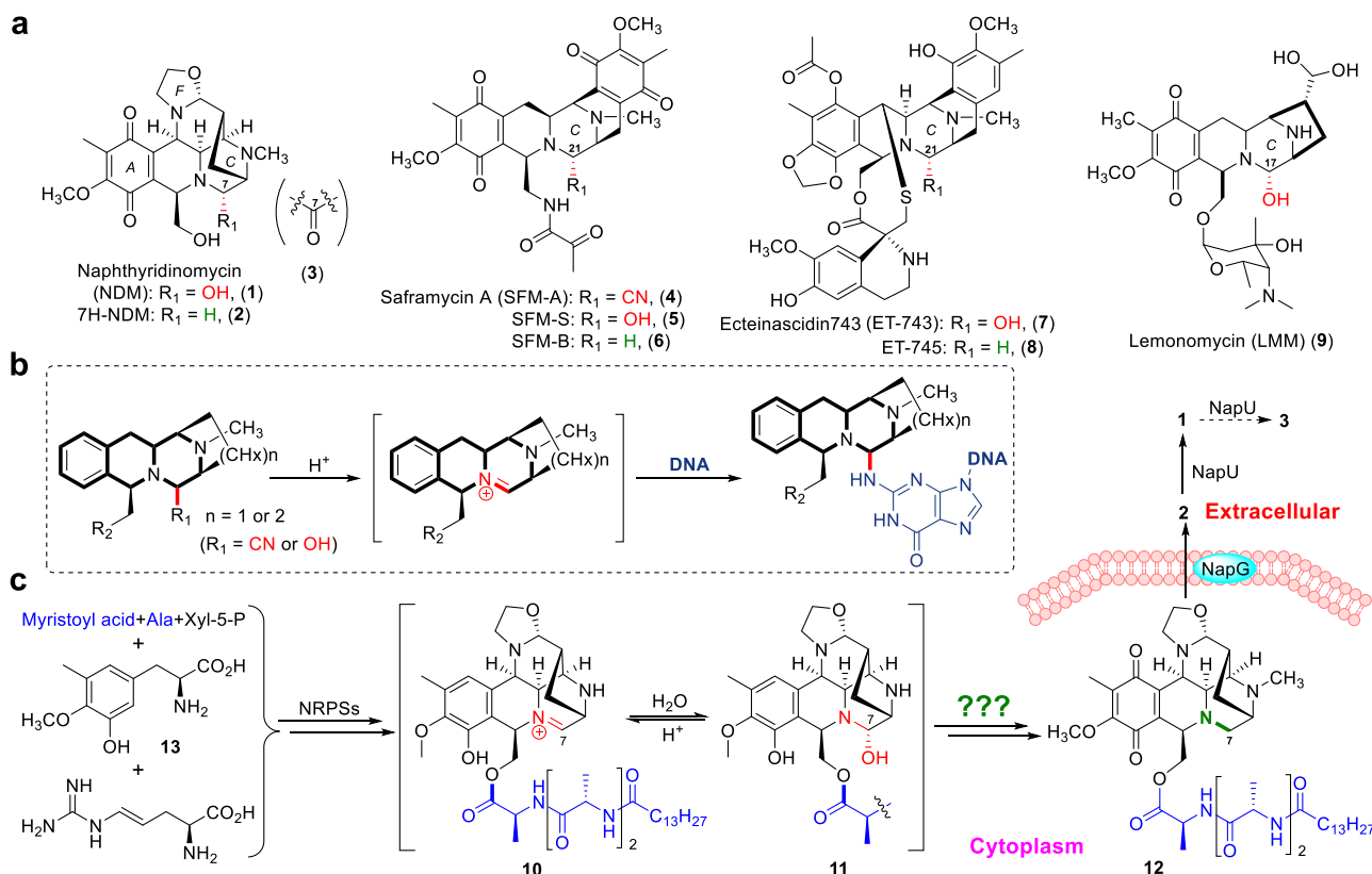
Fig. 1 Members of THIQ antibiotics, biosynthesis, and activation of NDM. a Chemical structures of typical THIQ antibiotics. b Proposed mechanism of THIQ antibiotic-mediated DNA alkylation. c Brief summary of NDM biosynthetic pathway featuring with intracellular pharmacophore quenching and extracellular reactivation.
