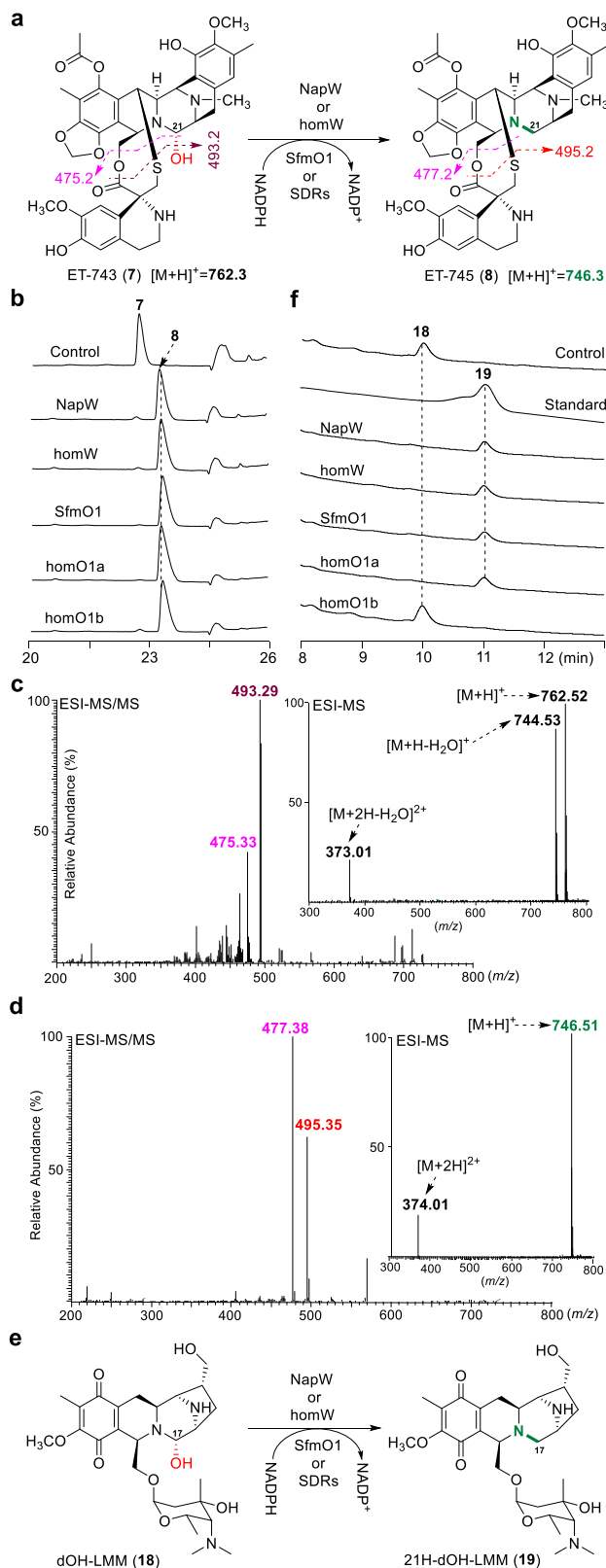
Fig. 6 Biochemical assay of SDRs-catalyzed reduction using ET-743 and dOH-LMM as substrates. SDRs-catalyzed reactions using 7 (a) or 18 (e) as substrate. HPLC analysis of enzymatic reactions with 7 (b) or 18 (f) as substrate. ESI-MS and ESI-MS/MS analysis of substrate 7 (c) and product 8 (d).
