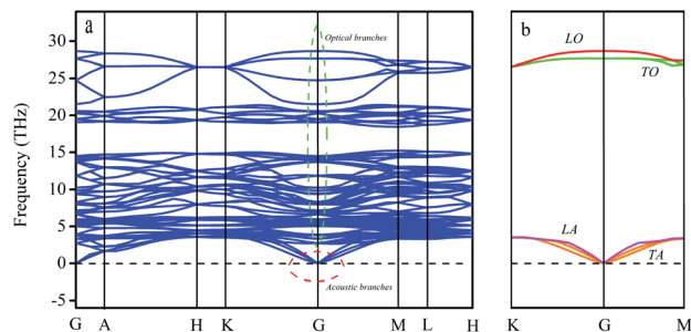
Fig. 4 The (a) phonon dispersion curves and (b) transverse & longitudinal waves in optics and acoustics of the R3c LaWN 3 structure.
