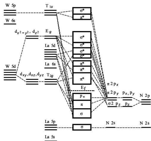
Fig. 5 Molecular-orbital bonding of LaWN 3 .
