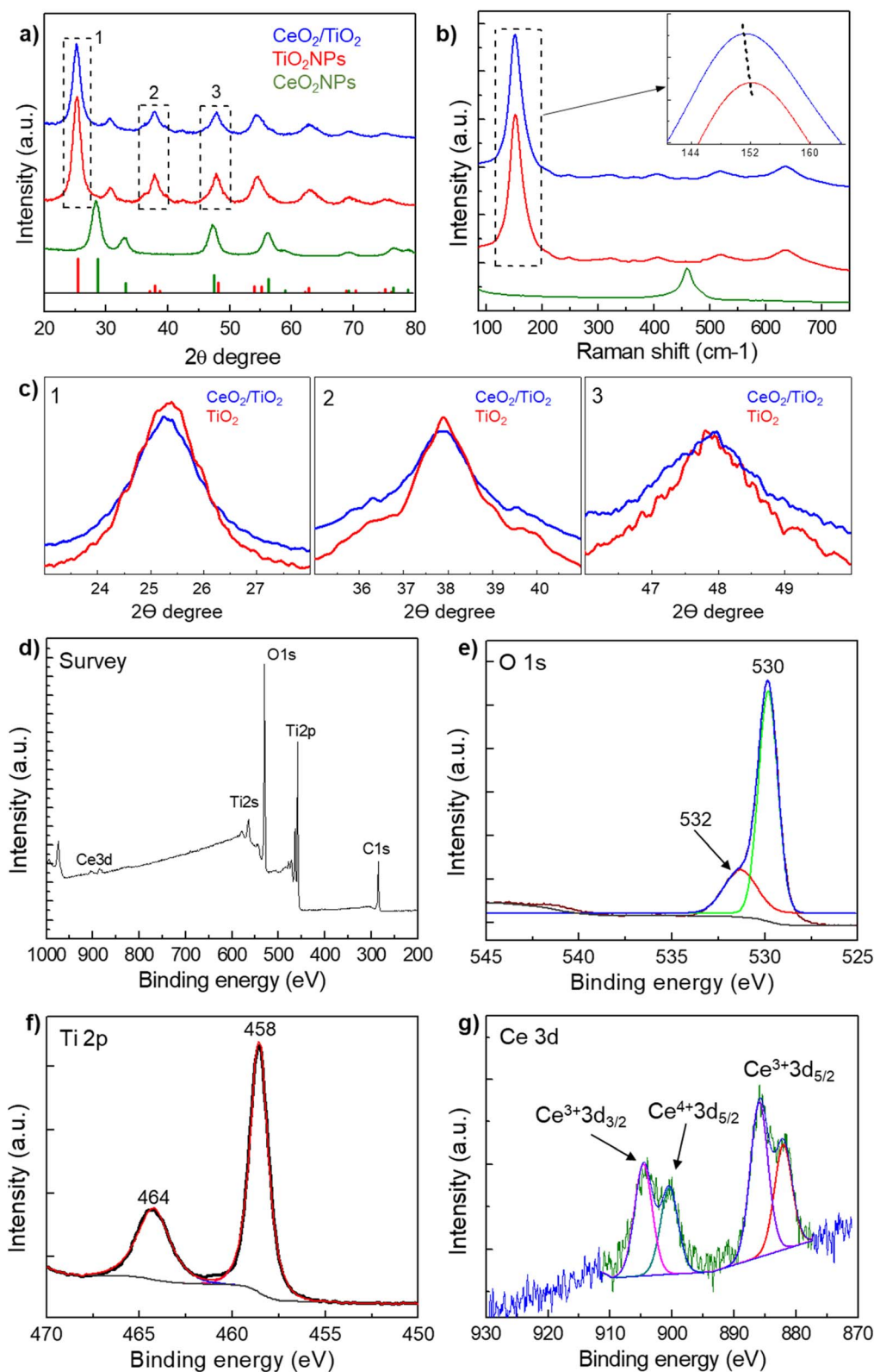
Fig. 2 Physicochemical characterization of the CeO 2 /TiO 2 hybrid nanostructures. (a) XRD patterns of the CeO 2 and TiO 2 NPs and the CeO 2 /TiO 2 hybrid. (b) Raman spectra of the CeO 2 and TiO 2 NPs and the CeO 2 /TiO 2 hybrid. Inset is the predominant peak of TiO 2 which is blue-shifted in the CeO 2 /TiO 2 hybrid. (c) Details of the anatase TiO 2 and CeO 2 /TiO 2 hybrid diffraction peaks at around 25° (1), 38° (2) and 48.0° (3). (d–g) XPS analysis of the CeO 2 /TiO 2 including survey spectra (d), O 1s core-level spectra (e), Ti 2p core-level spectra (f) and Ce 3d core-level spectra (g).
