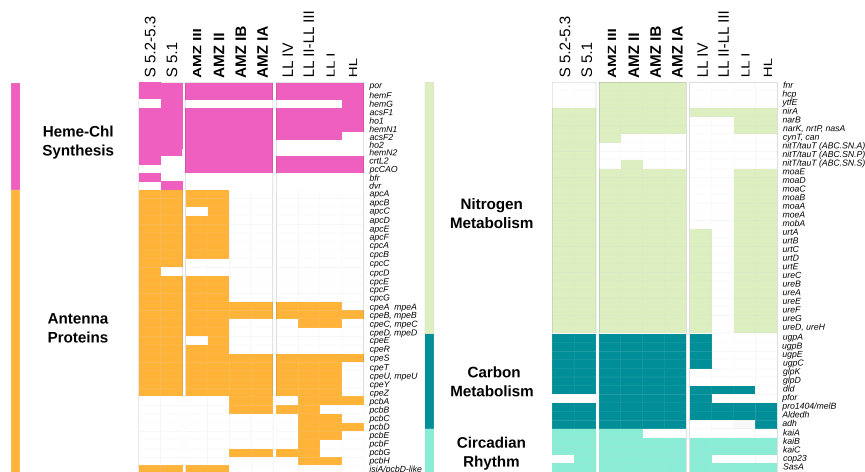
Fig. 2. Presence-absence of selected genes in AMZ Prochlorococcus SAGs (see SI Appendix, Tables S2 and S3 for details).
